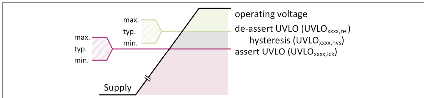
Figure 11 Voltage Monitoring
