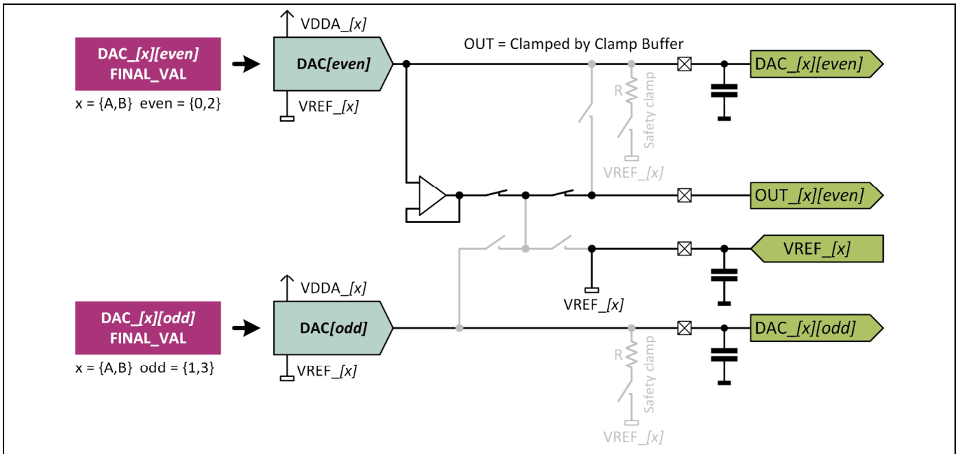
Figure 36 Clamping with Clamp Buffer
