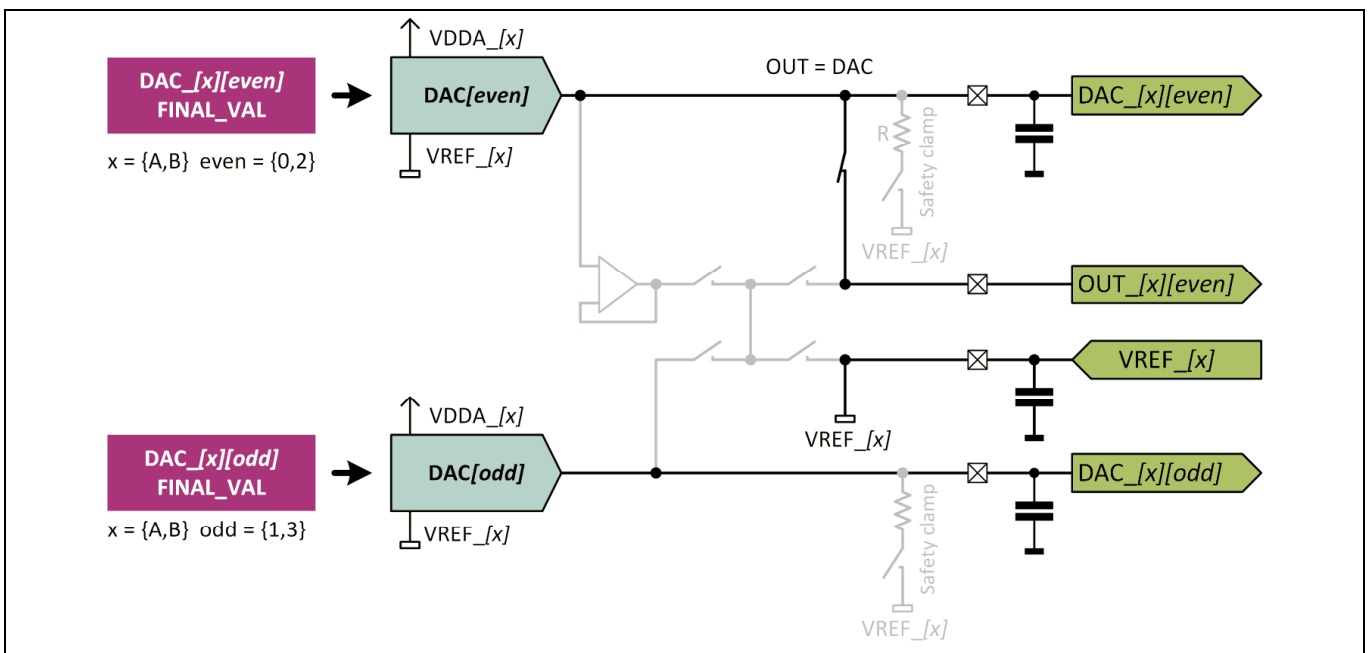
Figure 17 DAC and OUT Voltage in Active Mode
