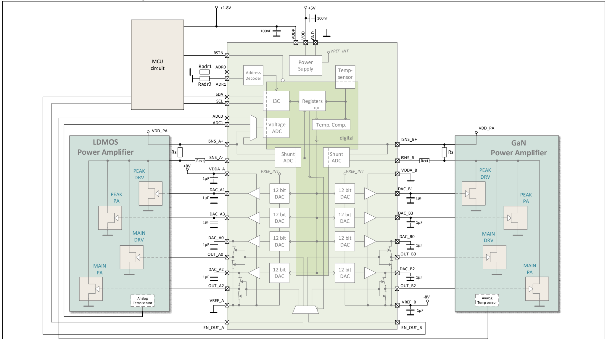
Figure 71 Typical application schematic circuit: biasing LDMOS and GaN Power Amplifiers
