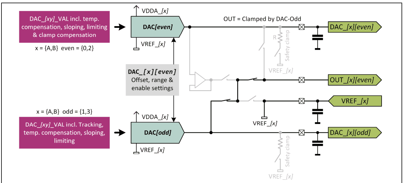
Figure 35 Clamping with Neighboring DAC
