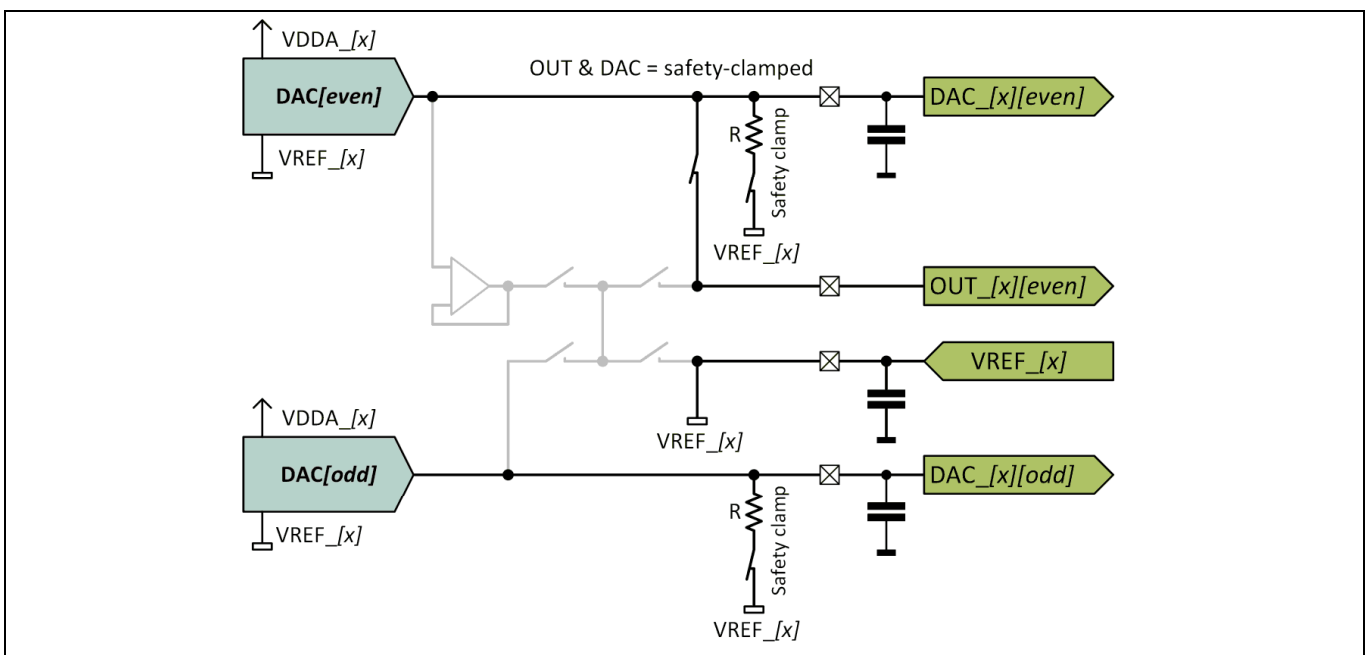
Figure 15 DAC Power-On / Reset Behavior
