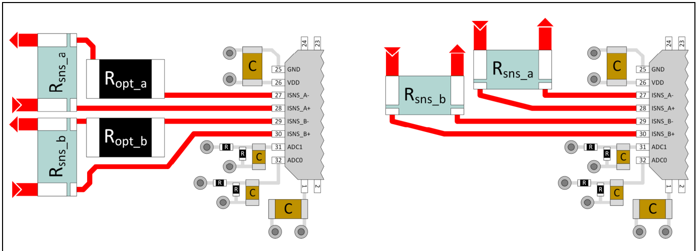
Figure 73 Reference Design Current Sense ADC
