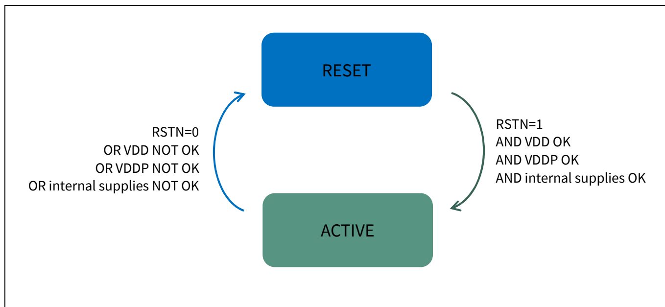
Figure 12 BGMC1210 state diagram
