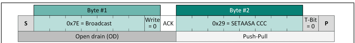
Figure 61 SETAASA Command Structure
