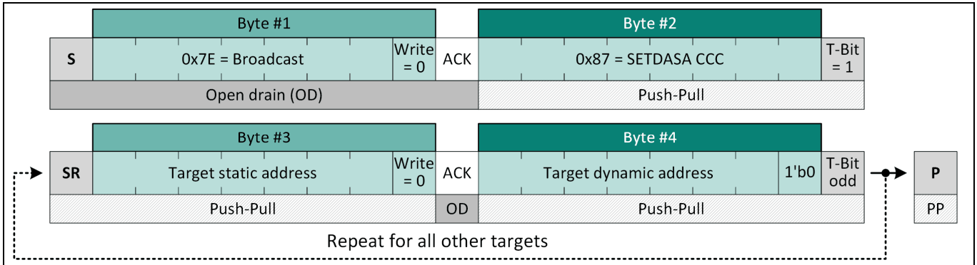
Figure 60 SETDASA Command Structure
