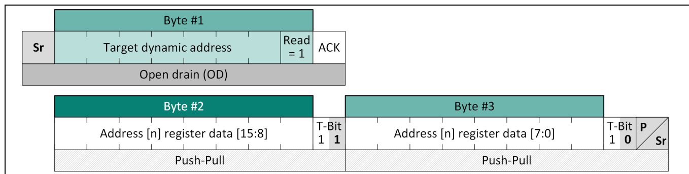
Figure 64 I3C SDR single read from current address
