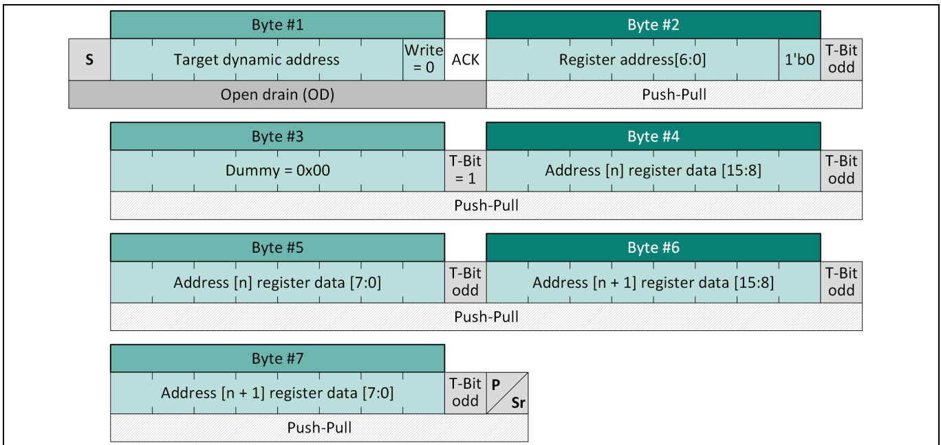
Figure 66 I3C SDR block write
