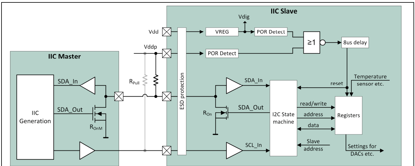
Figure 48 I2C Structure
