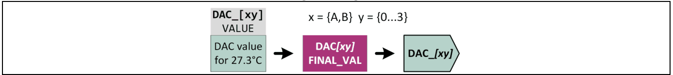
Figure 16 DAC Output Voltage Simple View
