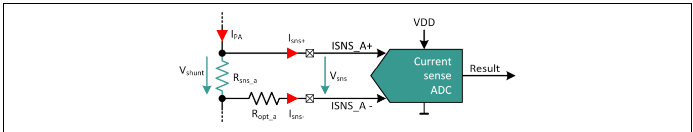
Figure 72 Reference Schematic Current Sense ADC
