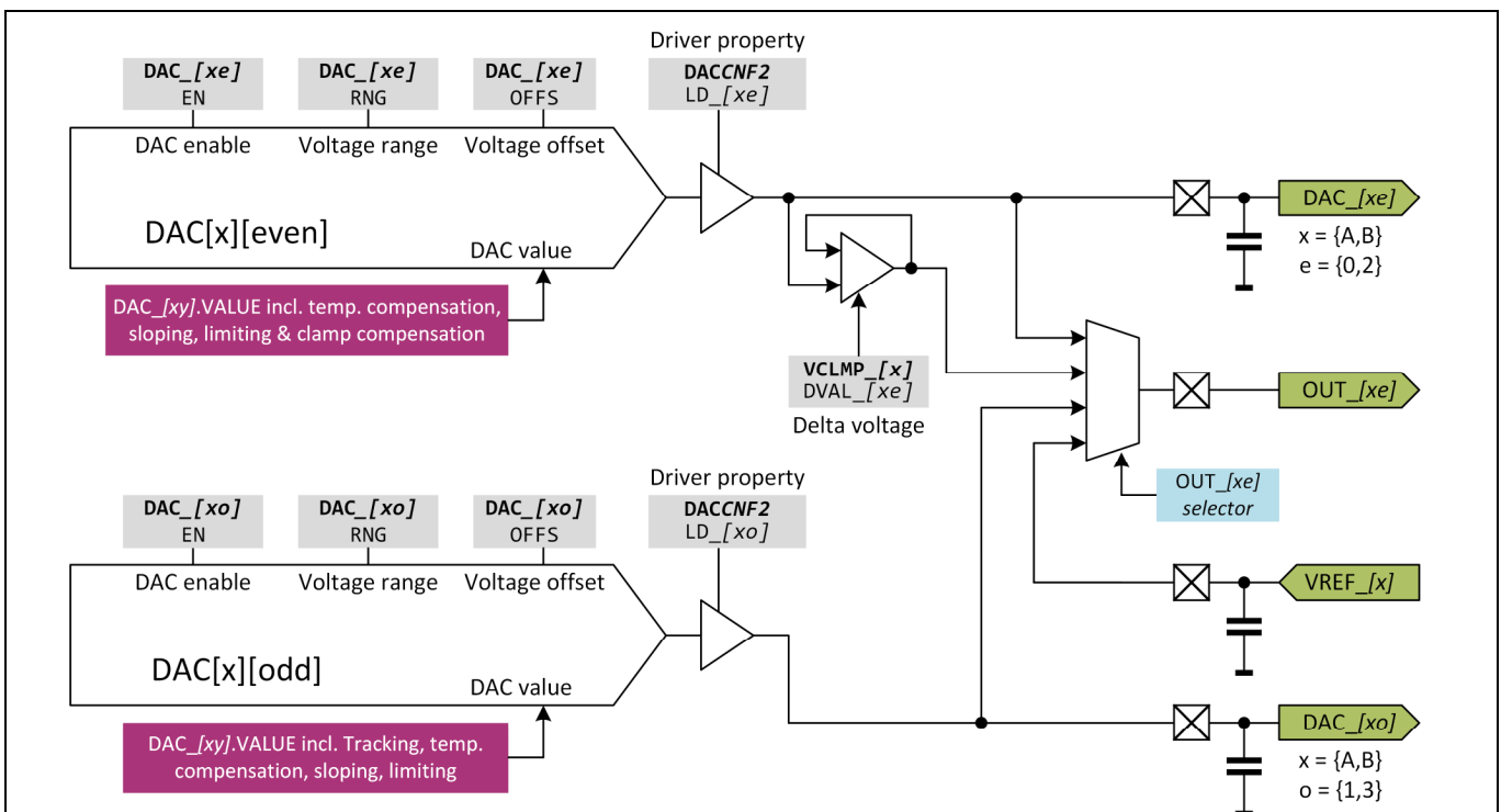
Figure 14 DACs And Their Registers
