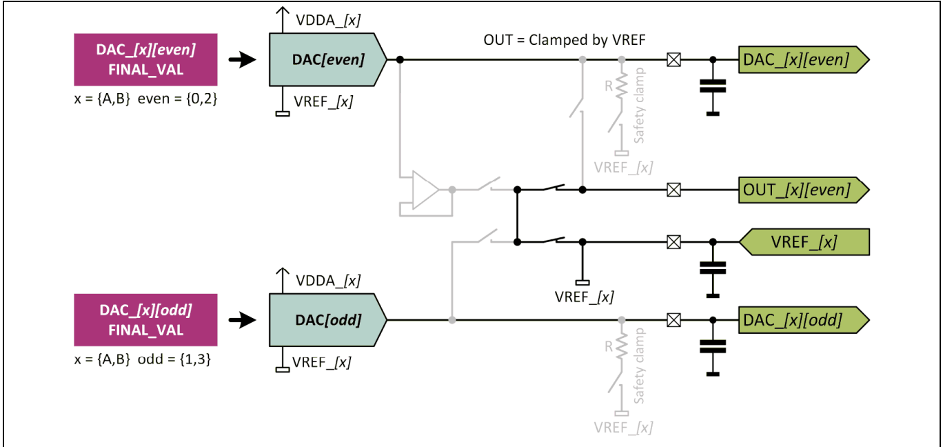
Figure 34 Clamping Using VREF
