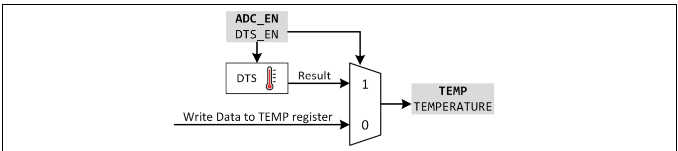
Figure 42 DTS Temperature Overwrite
