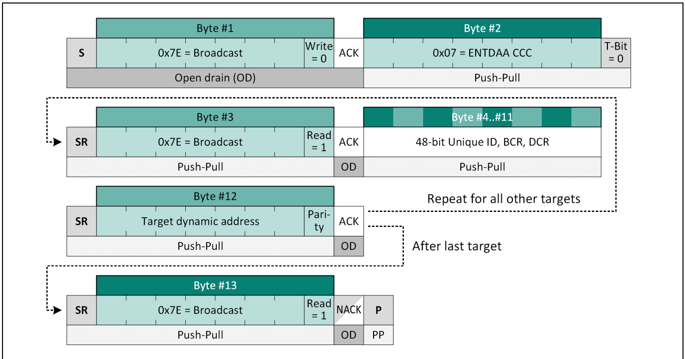
Figure 59 ENTDAAC Command Structure
