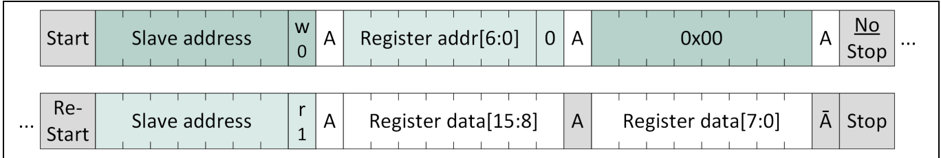
Figure 56 I2C Single Read Access
