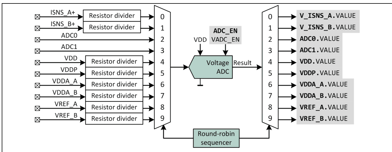
Figure 37 Voltage ADC
