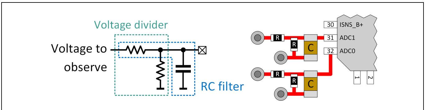
Figure 74 VADC reference circuit and layout
