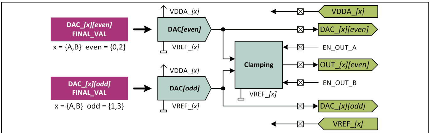
Figure 13 DAC Simplified Block Diagram
