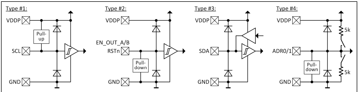
Figure 4 ESD protection for digital pins
