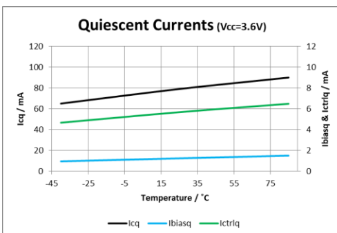
Figure 24: Quiescent Currents
