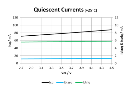
Figure 25: Quiescent Currents
