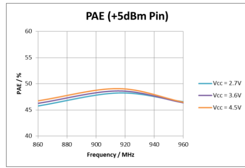
Figure 7: PAE (+5 dBm Pin)
