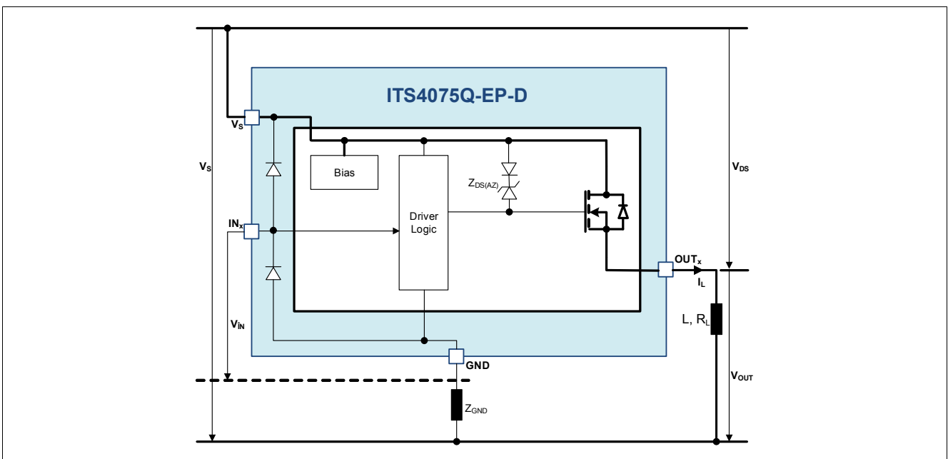
Figure 8 Output Clamp
