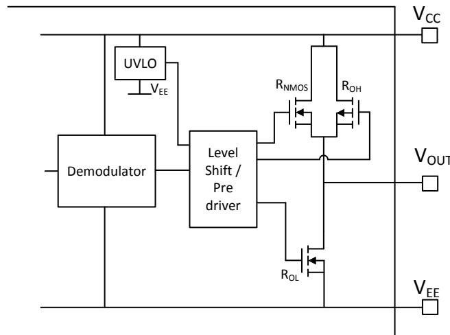
Figure 8-4. Output Stage
