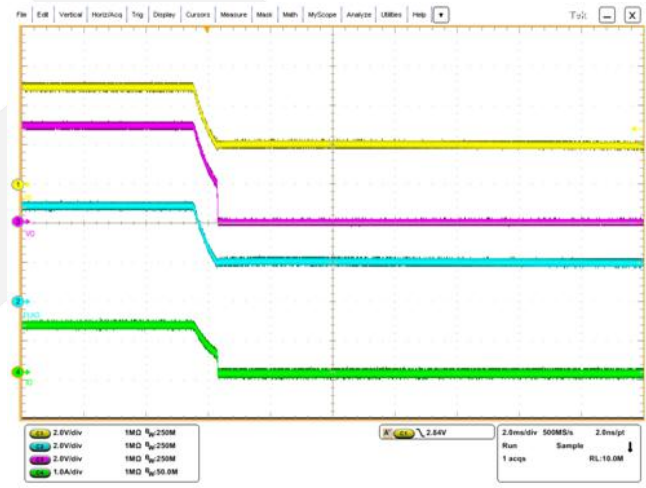
( V_{IN} = 5\text{ V} , V_{EN} = V_{IN} , R_{OUT} = 3.9\ \Omega , V_{IN} \rightarrow 0\text{ V} ) Figure 17. UVLO
