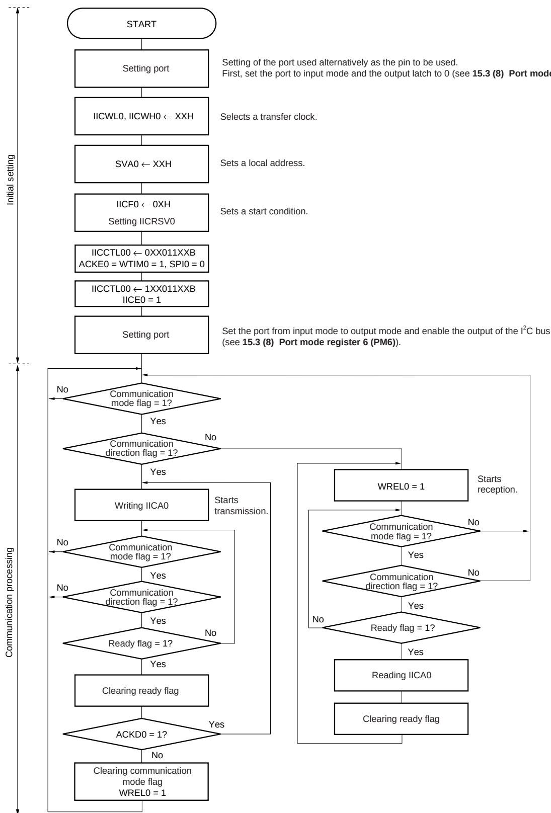
Figure 15-30. Slave Operation Flowchart (1)
