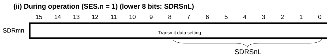
Figure 13-58. Example of Contents of Registers for Slave Transmission of 3-Wire Serial I/O (CSI S n) (2/2)
