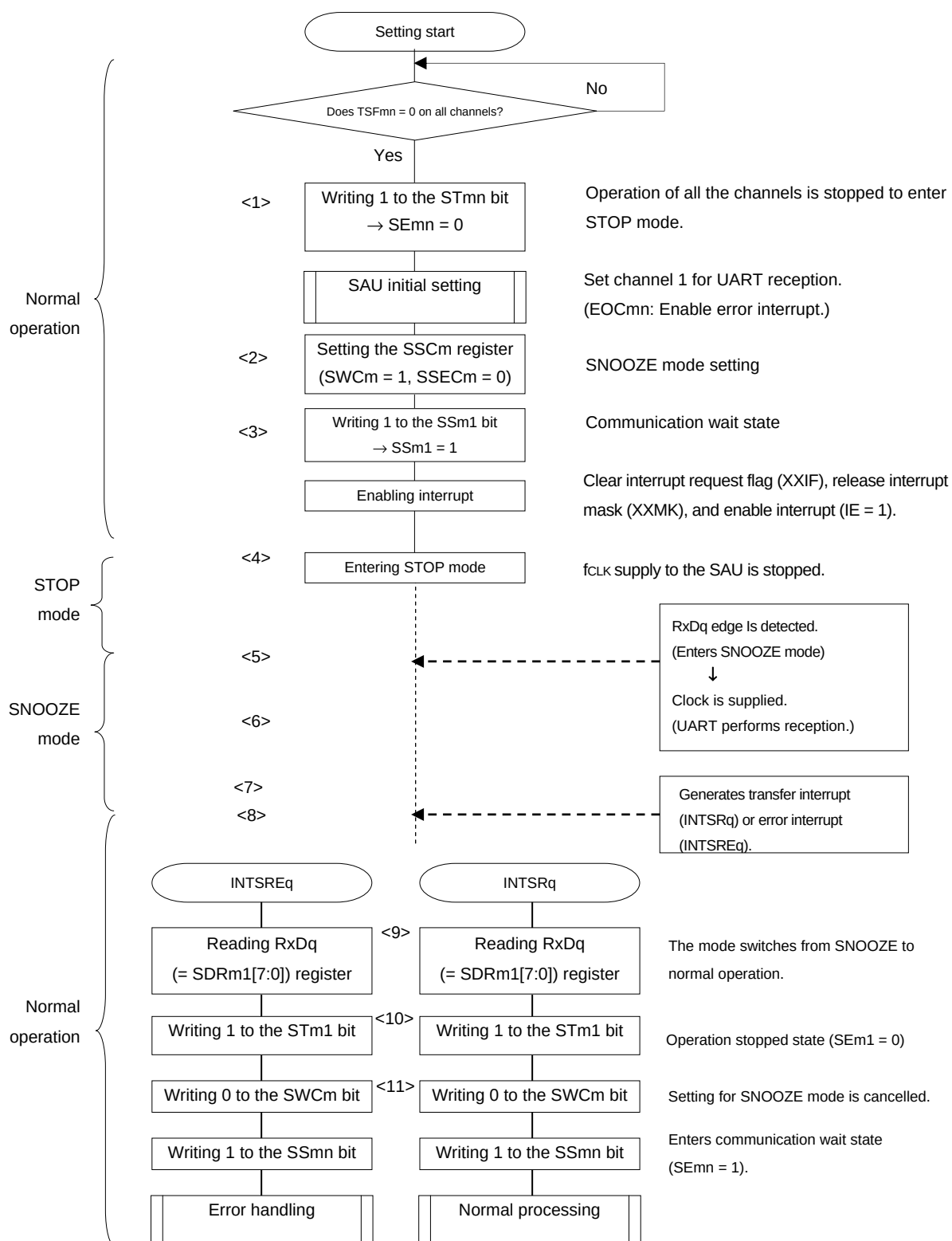
Figure 13-105. Flowchart of SNOOZE Mode Operation (Normal Operation/Abnormal Operation &lt;1&gt;)
