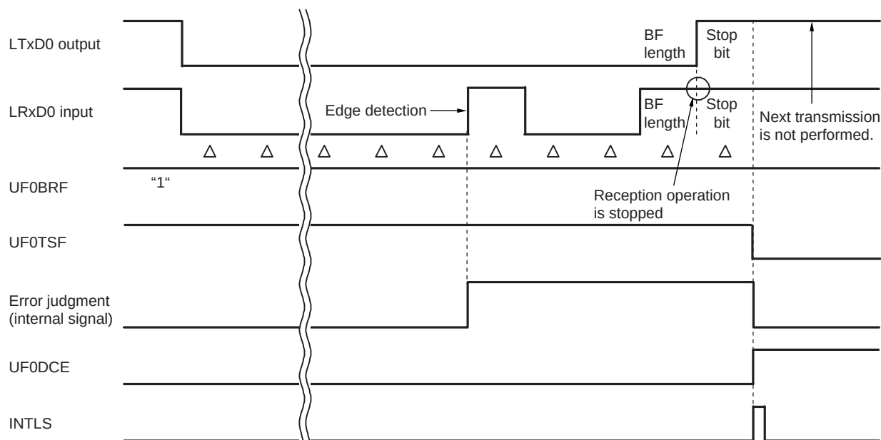
Figure 14-39. Timing of Occurrence of Data Consistency Error When BF Is Transmitted When UF0BRF = 1 (When Reception Is in Progress After Transmission of Stop Bit Has Stopped (Previous Input Data = 1))
