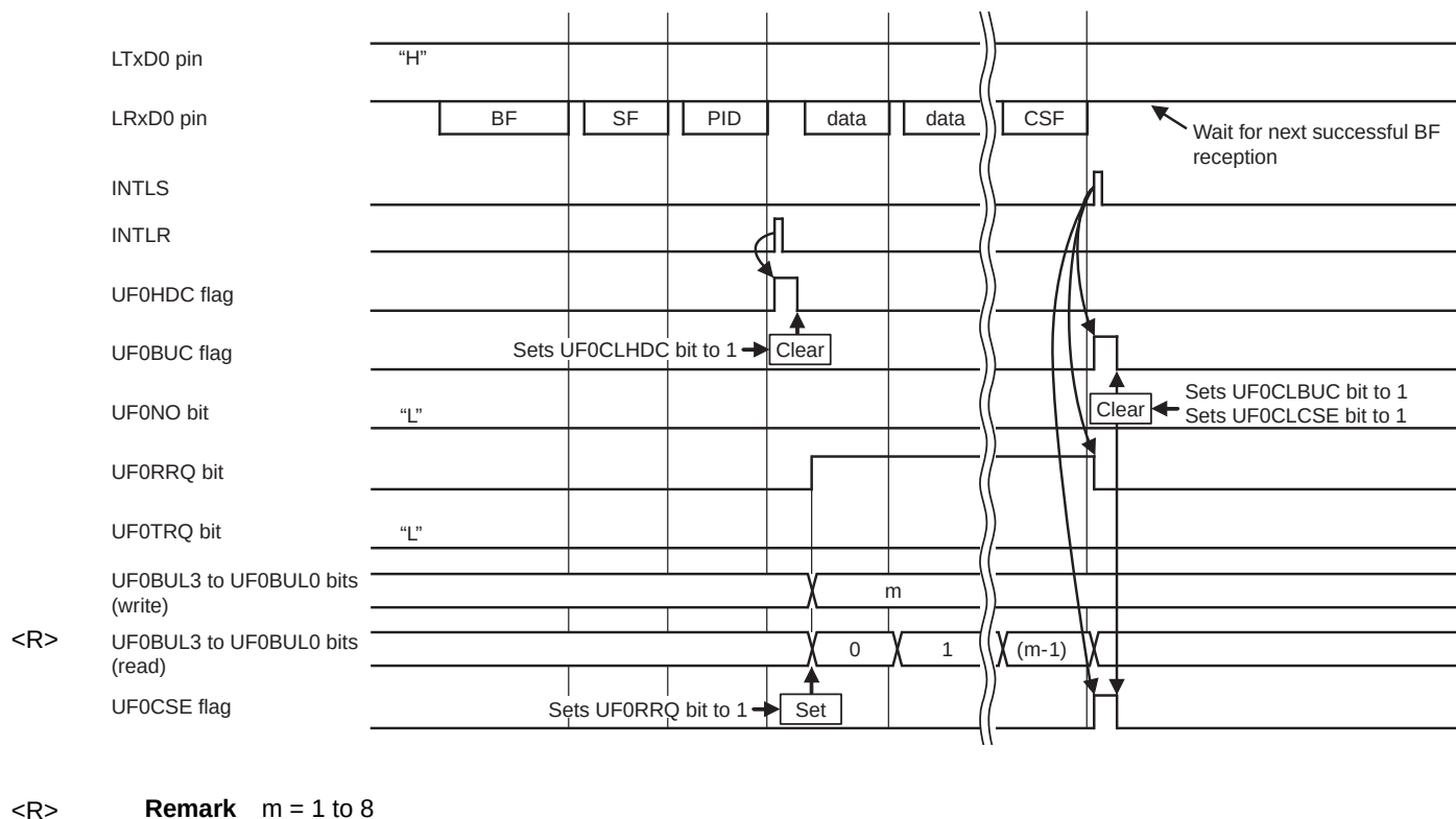
Figure 14-61. Automatic Checksum Error Occurrence Example (Response Reception)
