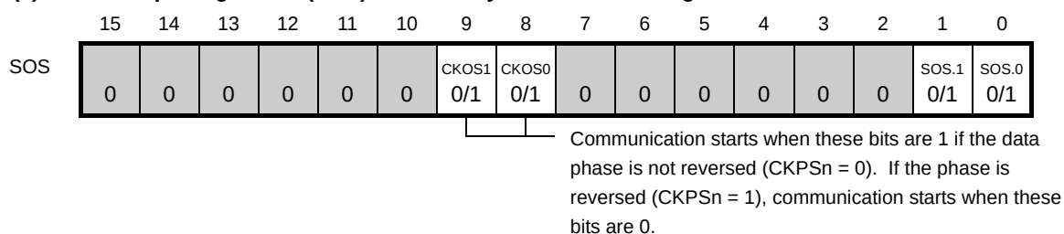
Figure 13-49. Example of Contents of Registers for Master Transmission/Reception of 3-Wire Serial I/O (CSISn) (1/2)
