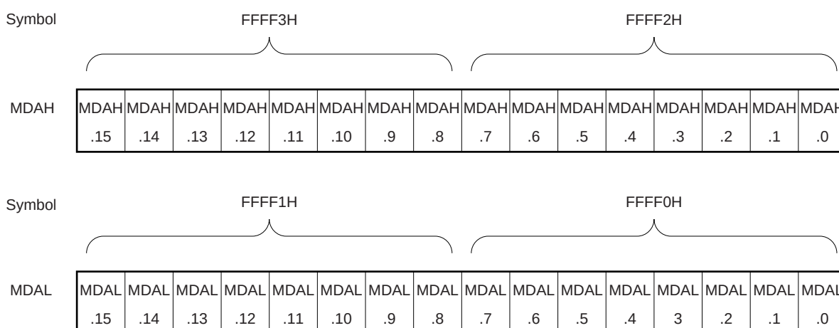
Figure 16-2. Format of Multiplication/Division Data Register A (MDAH, MDAL)
