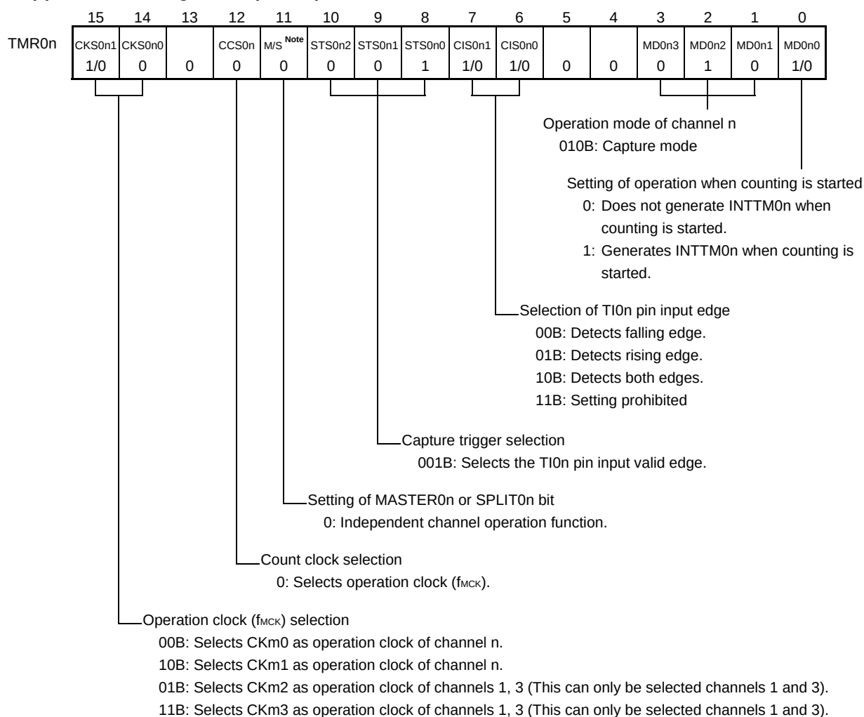
Figure 6-62. Example of Set Contents of Registers to Measure Input Pulse Interval
