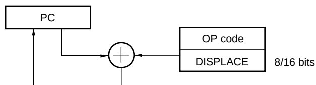
Figure 3-20. Outline of Relative Addressing
