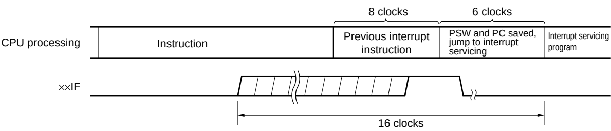
Figure 18-9. Interrupt Request Acknowledgment Timing (Maximum Time)
