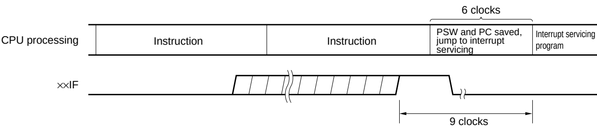
Figure 18-8. Interrupt Request Acknowledgment Timing (Minimum Time)
