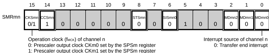
Figure 13-66. Example of Contents of Registers for Slave Reception of 3-Wire Serial I/O (CSI00, CSI01, CSI10, CSI11, CSI20, CSI21)
