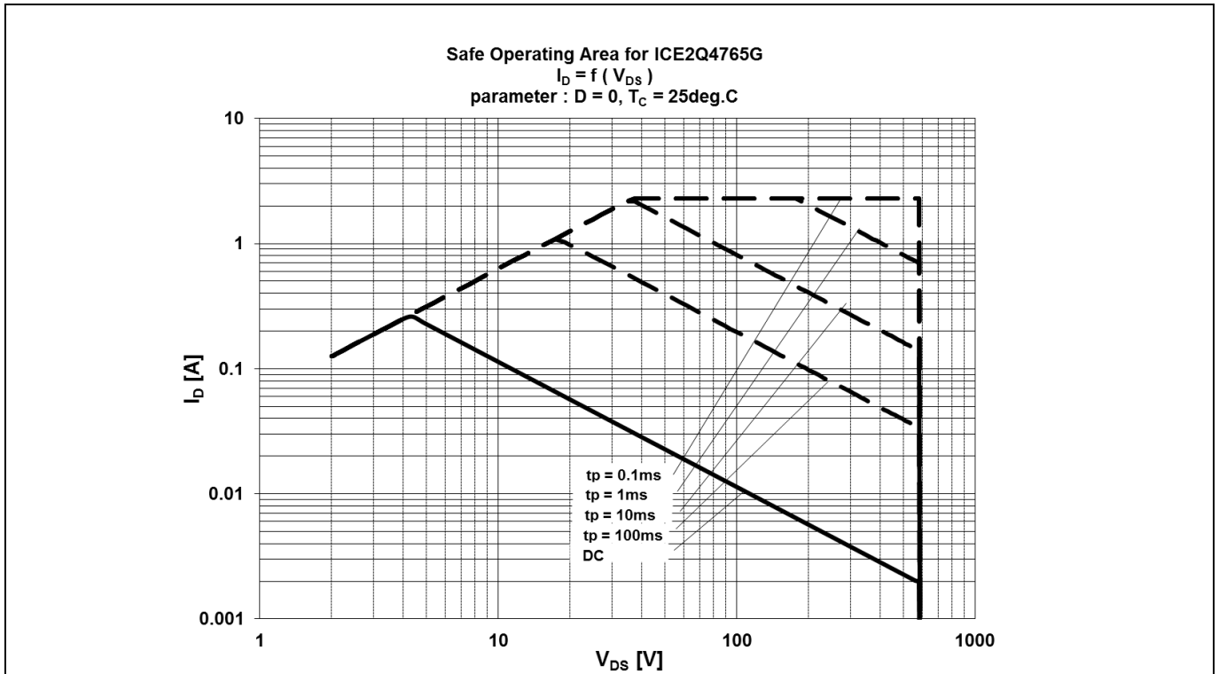
Figure 10 Safe Operating Area (SOA) curve for ICE2QR4765G
