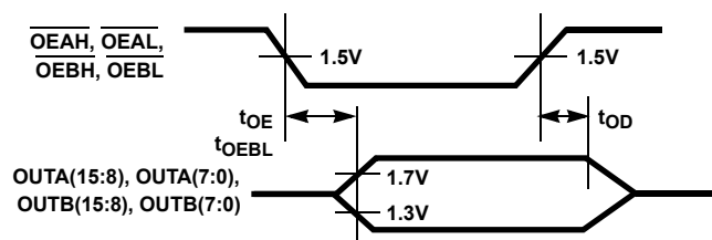
FIGURE 53. OUTPUT ENABLE/DISABLE
