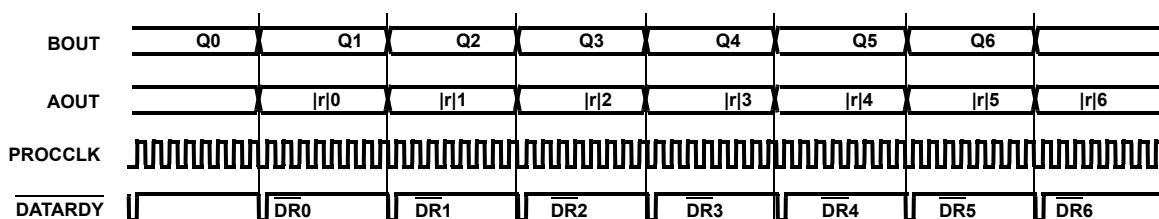
FIGURE 32. \overline{\text{DATARDY}} WAVEFORMS WHEN |r| (MAGNITUDE) IS SELECTED AS AOUT
