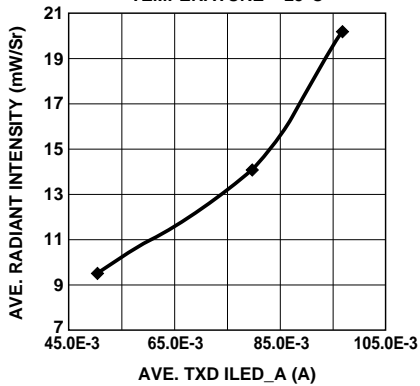
AVE. TXD RADIANT INTENSITY vs. AVE. TXD ILED_A, TEMPERATURE = 25°C
