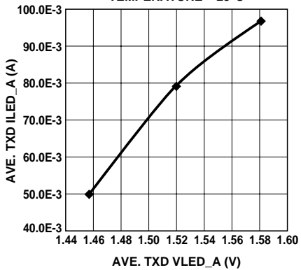
AVE. TXD ILED_A vs. AVE. TXD VLED_A, TEMPERATURE = 25°C
