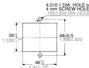
Rear surface-mounting
