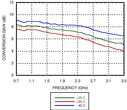
+2RF -2LO Response vs. Temperature @ VGATE=4.9V
