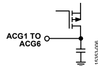
Figure 6. ACGx Pin Interface Schematic
