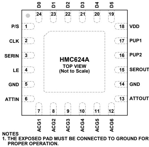
Figure 3. Pin Configuration
