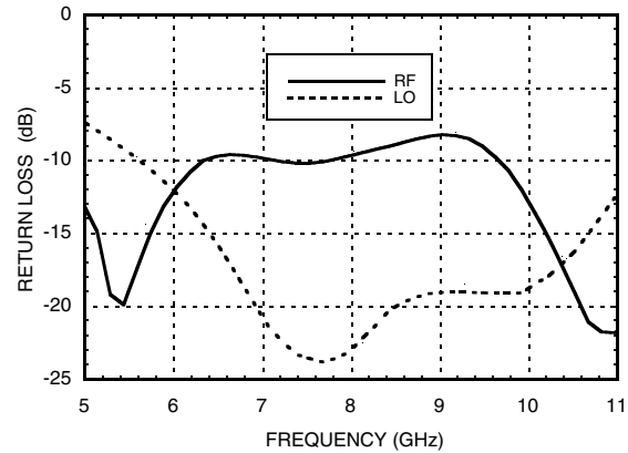
Return Loss
