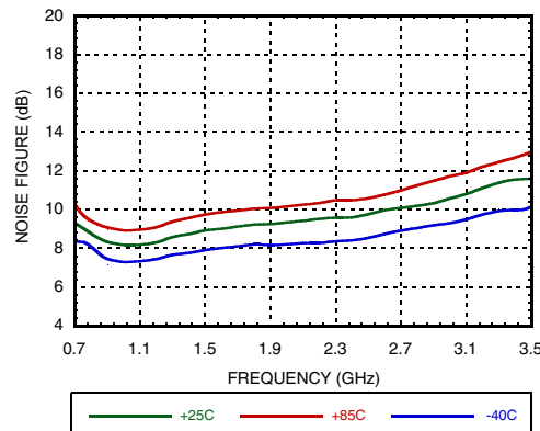
Figure 31. Noise Figure vs. Temperature @ VGATE=4.8V
