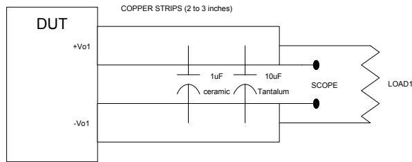
Figure 9. Output Ripple and Noise Measurement Test Setup
