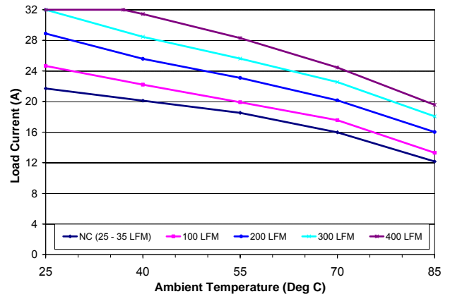
Figure 17. HKS Power Derating Curves
