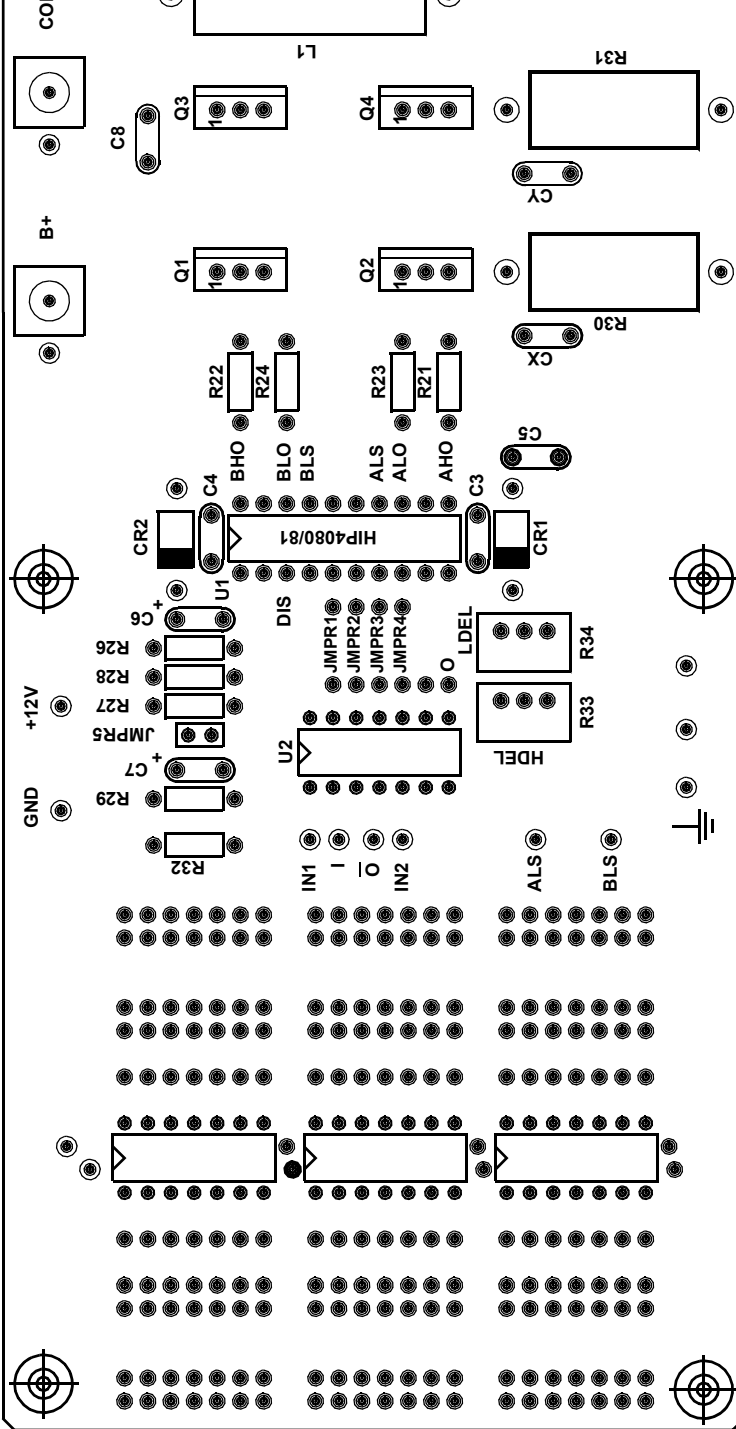
FIGURE 32. HIP4081A EVALUATION BOARD SILKSCREEN
