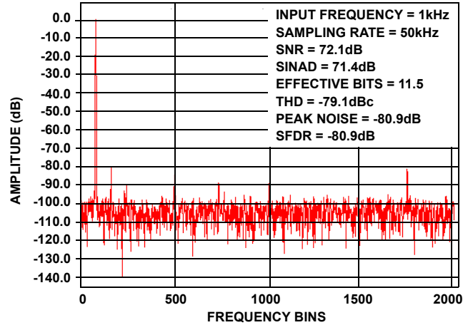
FIGURE 13. FFT SPECTRUM
