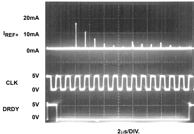
FIGURE 20. TYPICAL REFERENCE INPUT CURRENT
