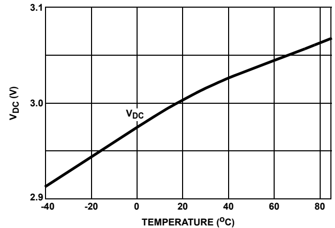
FIGURE 11. DC BIAS VOLTAGE ( V_{DC} ) vs TEMPERATURE
