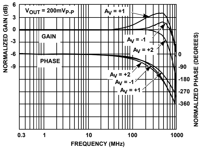
FIGURE 9. FREQUENCY RESPONSE
