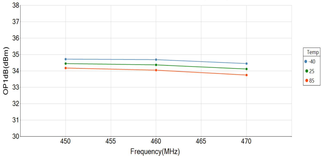
GRF5504 OP1dB vs Frequency
