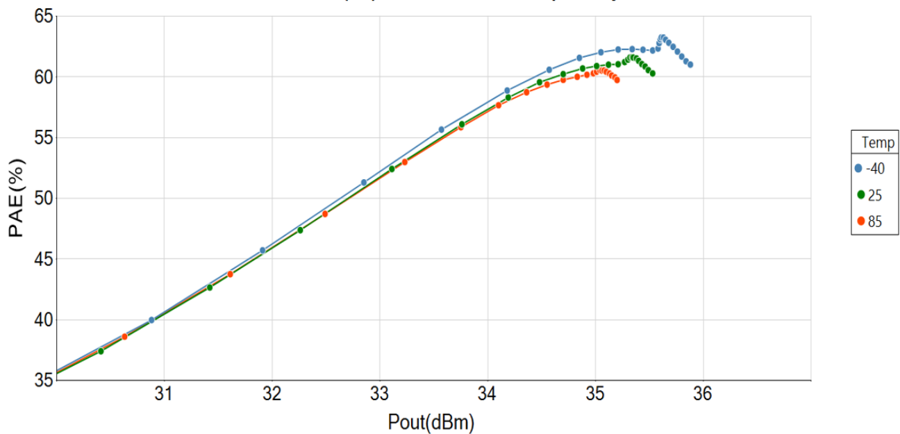
GRF5504 PAE(%) vs Pout at Frequency = 460 MHz
