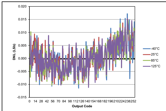
FIGURE 46-104: Typical DAC DNL Error, VDD = 5.0V, VREF = External 5.0V, PIC18F25/26K83 Only.
