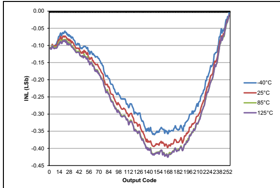
FIGURE 46-103: Typical DAC INL Error, VDD = 3.0V, VREF = External 3.0V.
