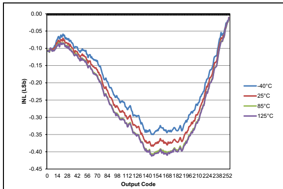
FIGURE 46-105: Typical DAC INL Error, VDD = 5.0V, VREF = External 5.0V PIC18F25/26K83 Only.
