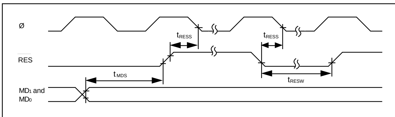
Figure 15-7. Reset Input Timing
