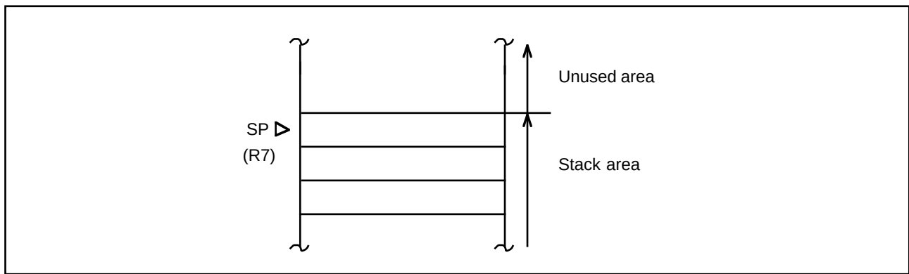
Figure 3-2. Stack Pointer
