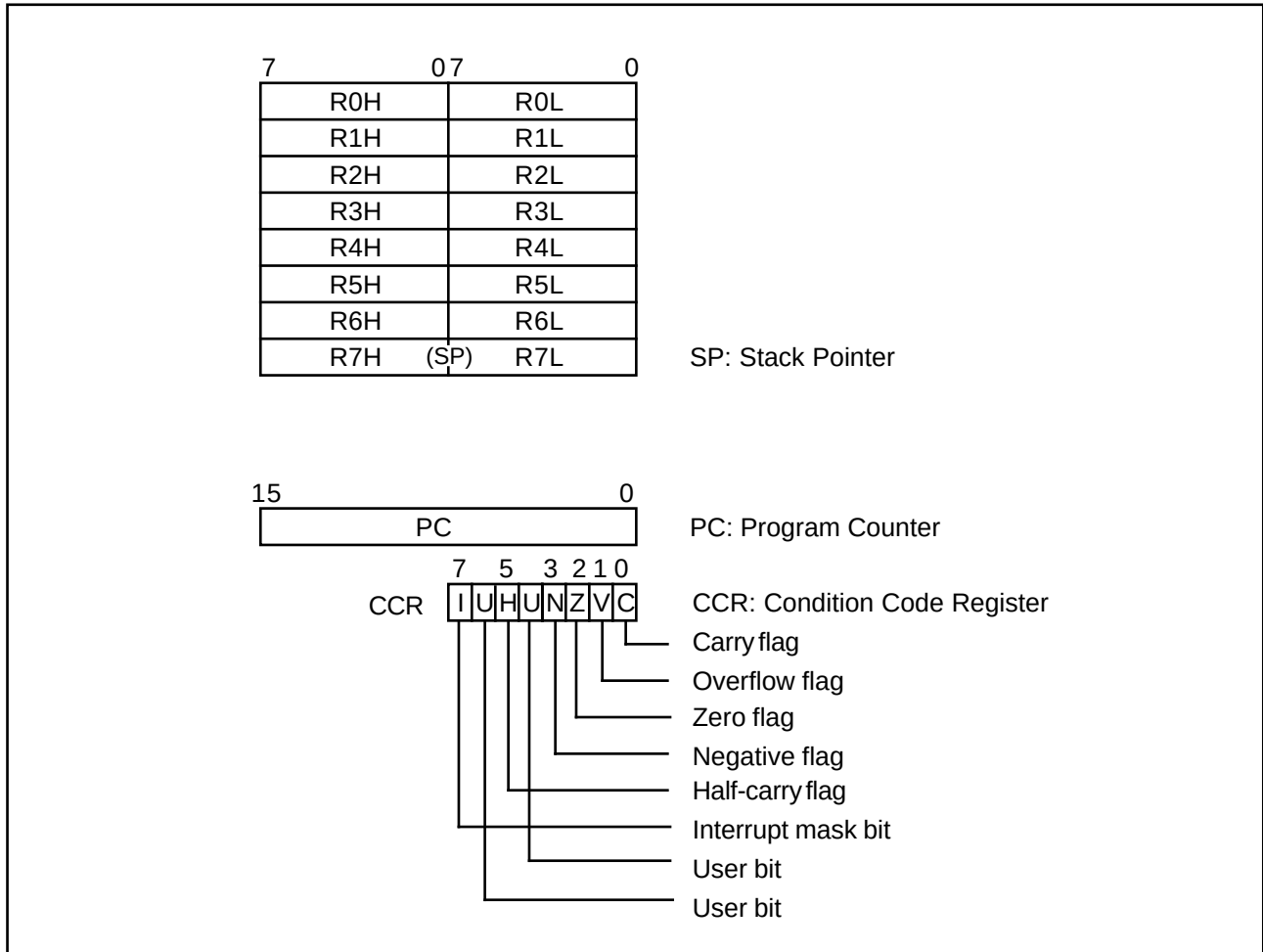
Figure 3-1. CPU Registers
