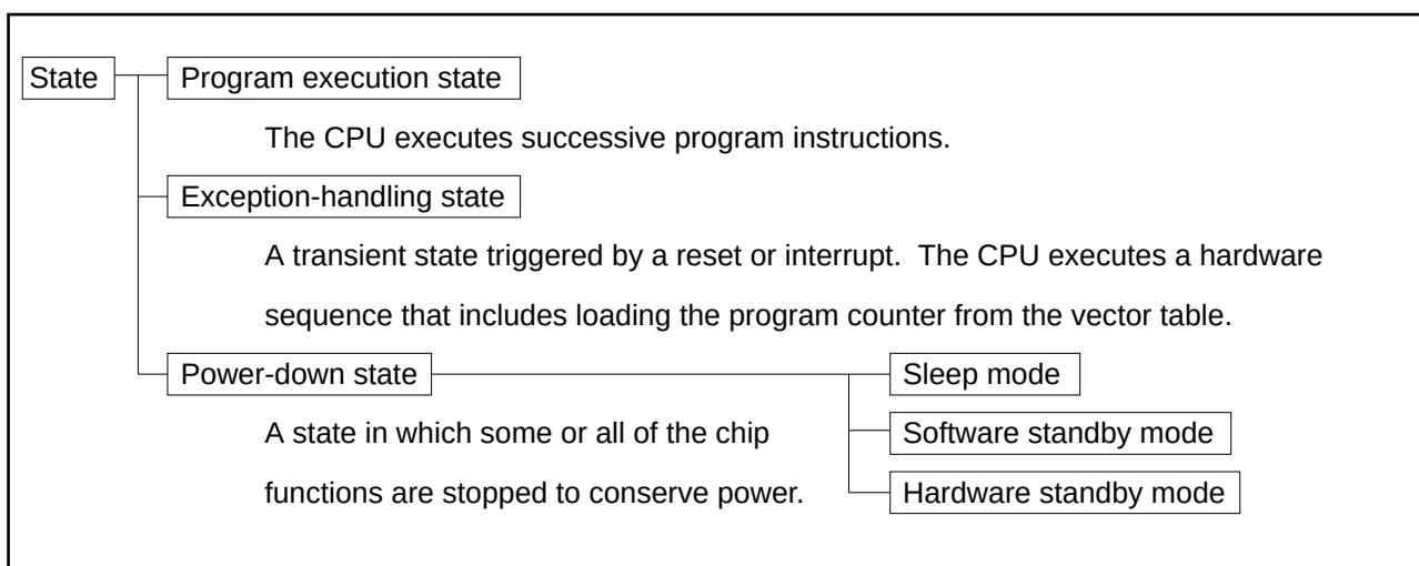
Figure 3-11. Operating States
