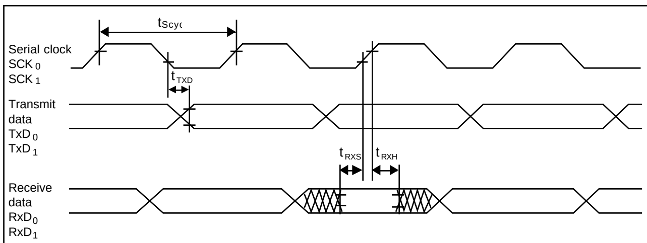
Figure 15-16. SCI Input/Output Timing (Synchronous Mode)
