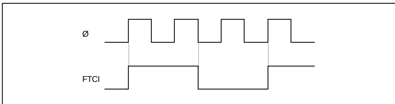
Figure 7-6. Minimum External Clock Pulse Width
