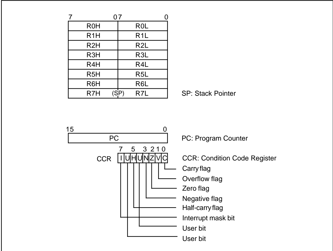
Figure 3-1. CPU Registers
