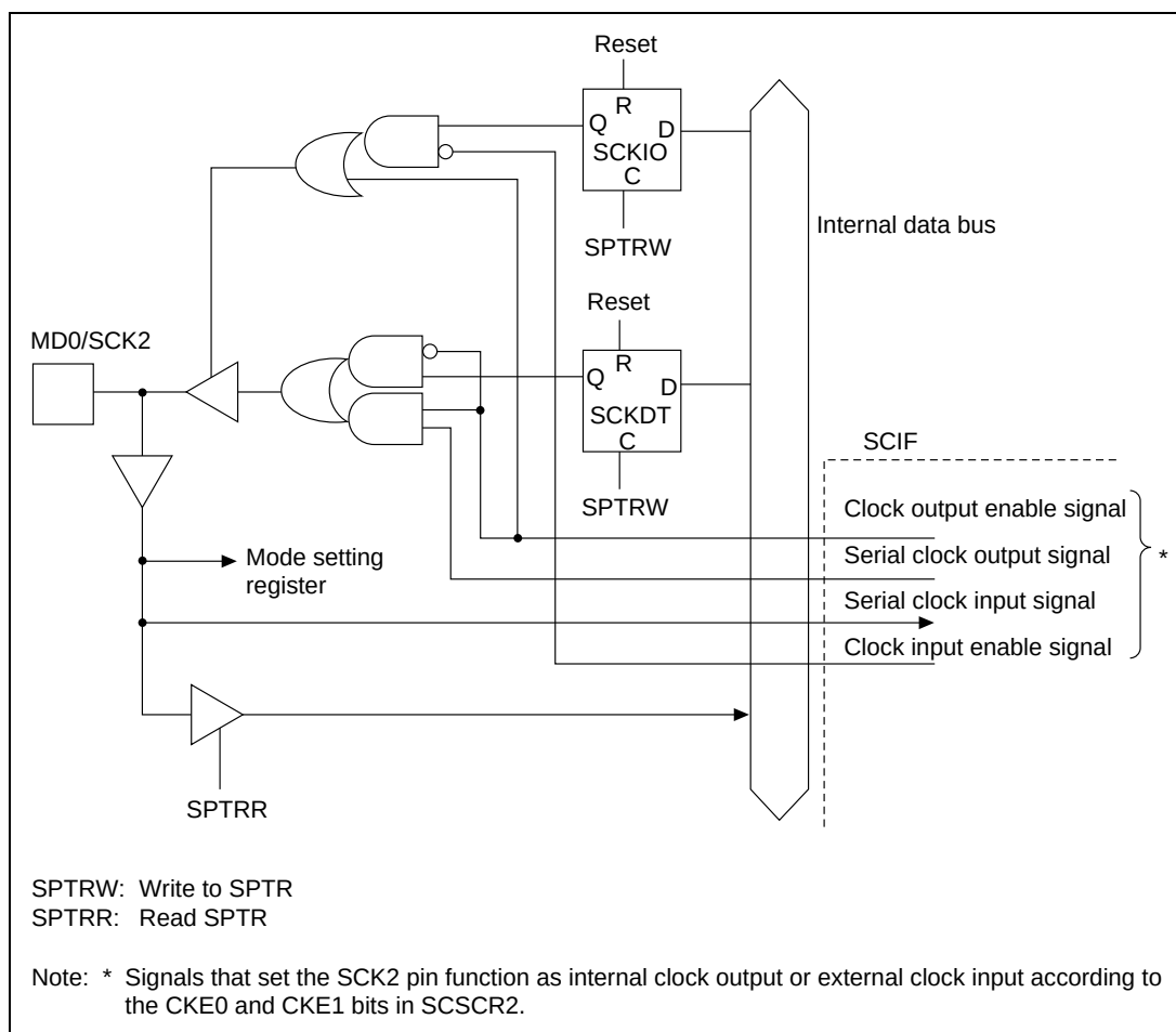
Figure 16.6 MD0/SCK2 Pin
