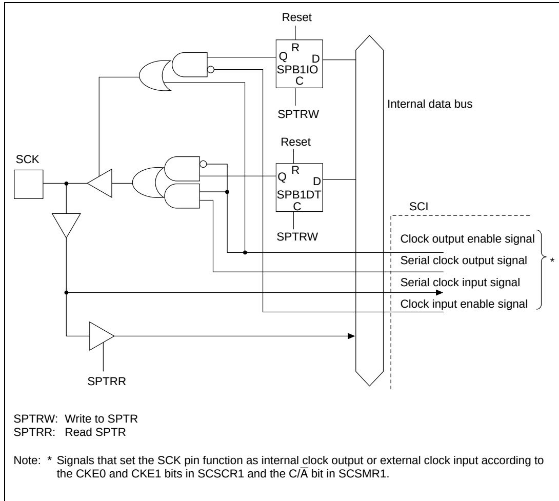
Figure 15.2 SCK Pin
