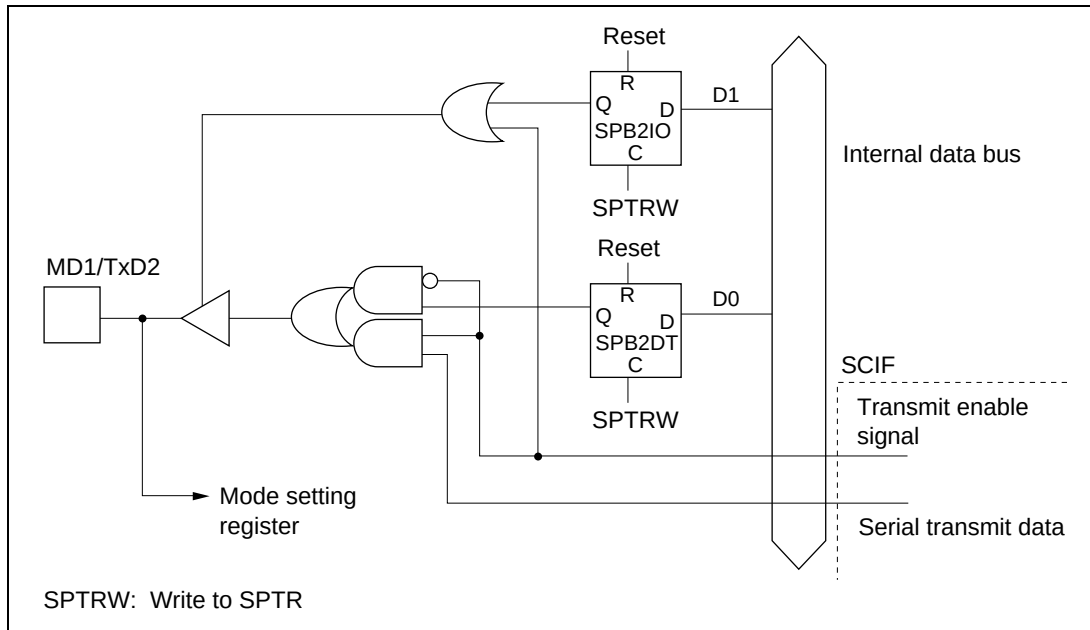
Figure 16.4 MD1/TxD2 Pin
