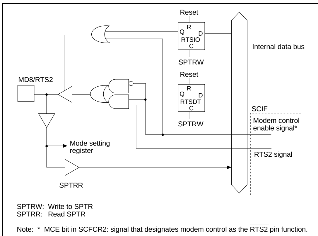
Figure 18.10 MD8/RTS2 Pin
