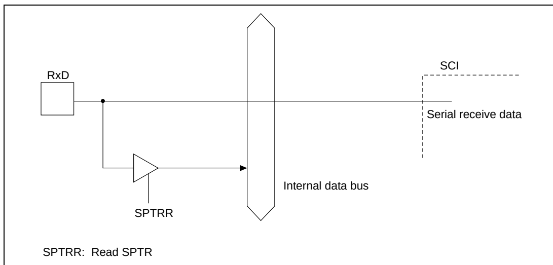
Figure 15.4 RxD Pin
