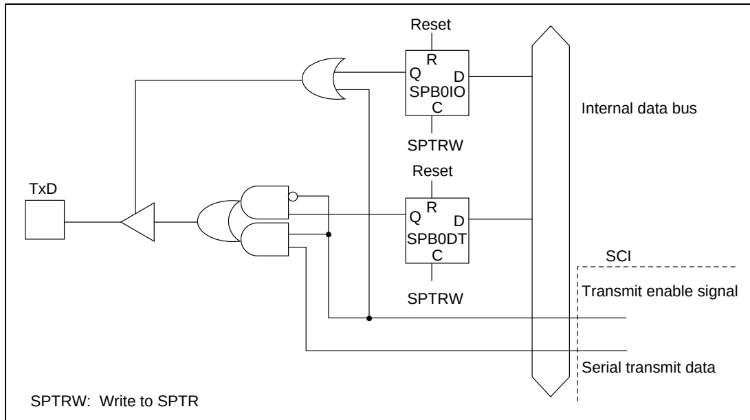
Figure 15.3 TxD Pin
