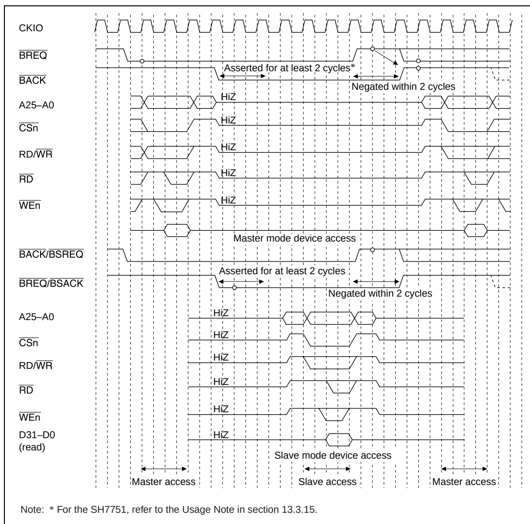
Figure 13.73 Arbitration Sequence
