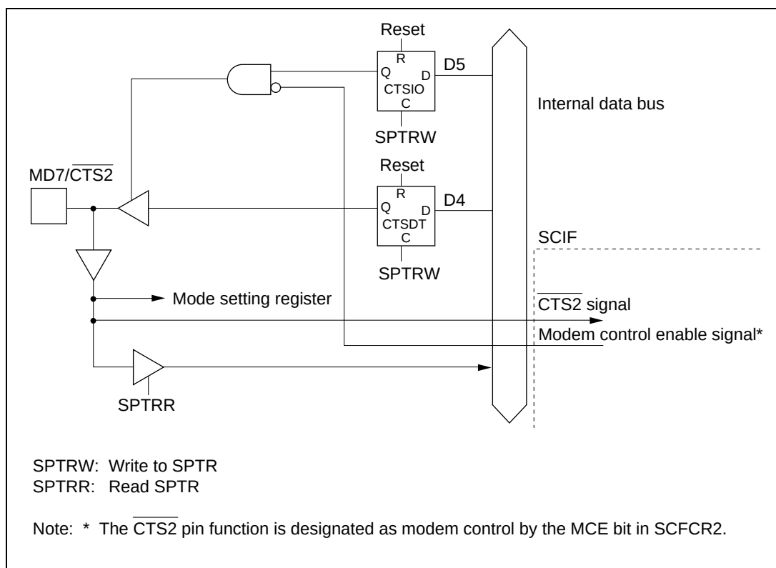
Figure 16.3 MD7/CTS2 Pin
