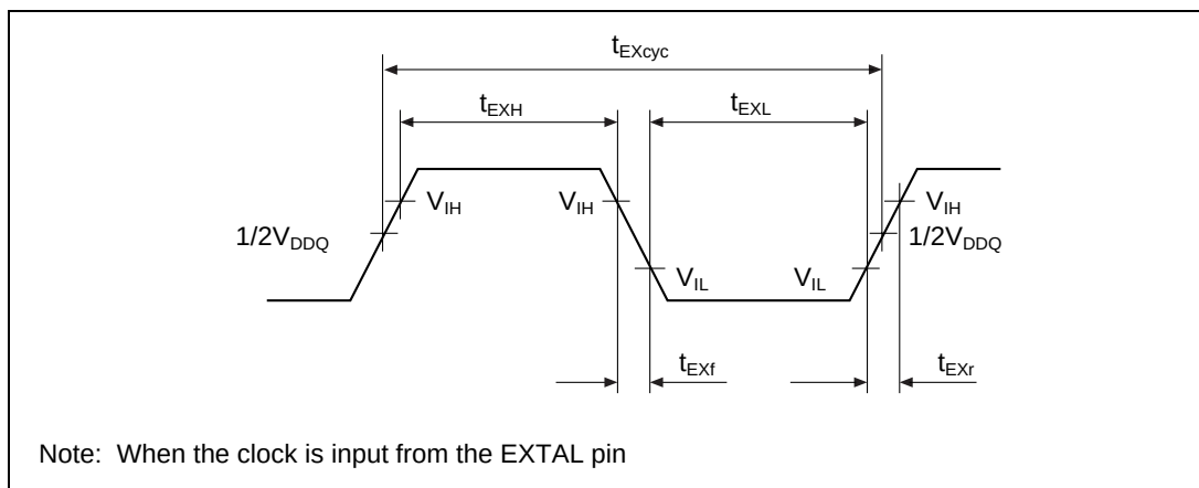
Figure 23.1 EXTERNAL Clock Input Timing
