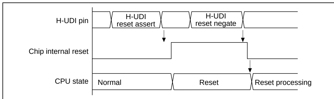
Figure 21.3 H-UDI Reset
