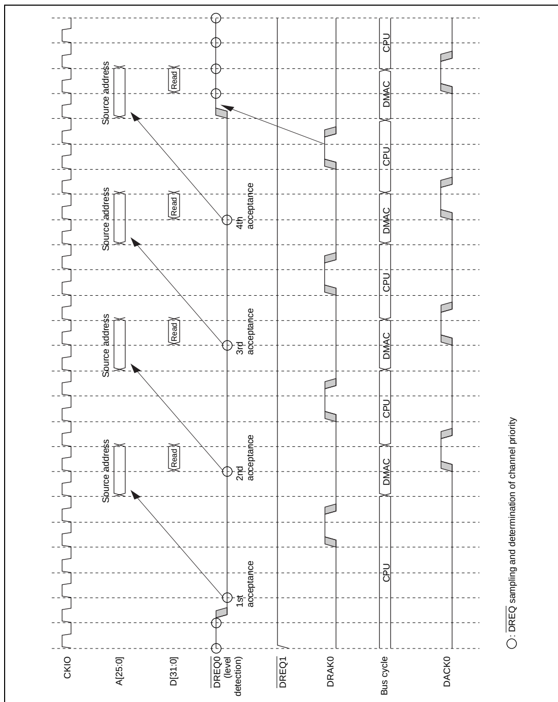
Figure 14.18 Single Address Mode/Cycle Steal Mode External Bus → External Bus/DREQ (Level Detection)
