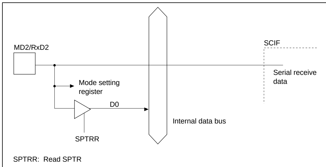
Figure 16.5 MD2/RxD2 Pin
