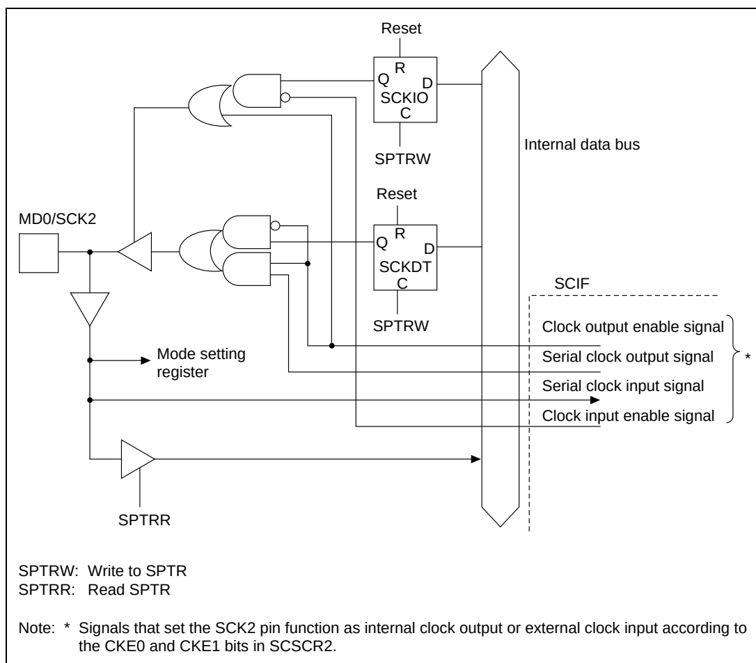
Figure 18.8 MD0/SCK2 Pin
