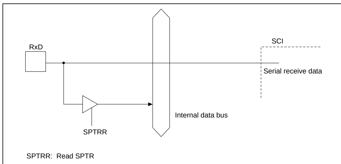
Figure 18.5 Rx D Pin
