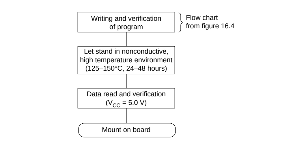
Figure 16.6 Screening Flow
