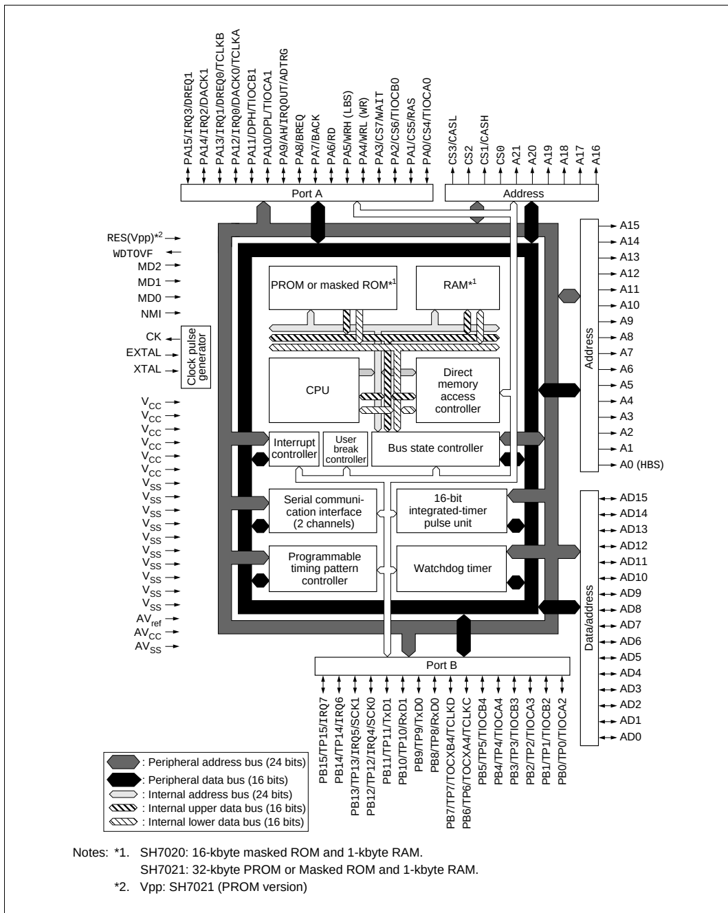
Figure 1.1 Block Diagram
