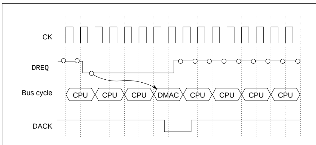
Figure 9.15 \overline{\text{DREQ}} Sampling Timing in Cycle Steal Mode (Output with \overline{\text{DREQ}} level detection and \text{DACK} active low) (Single address mode, bus cycle = 2 states)
