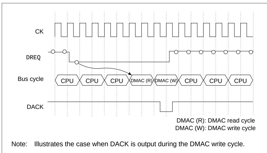
Figure 9.16 \overline{\text{DREQ}} Sampling Timing in Cycle Steal Mode (Output with \overline{\text{DREQ}} level detection and \text{DACK} active low) (Dual address mode, bus cycle = 2 states)
