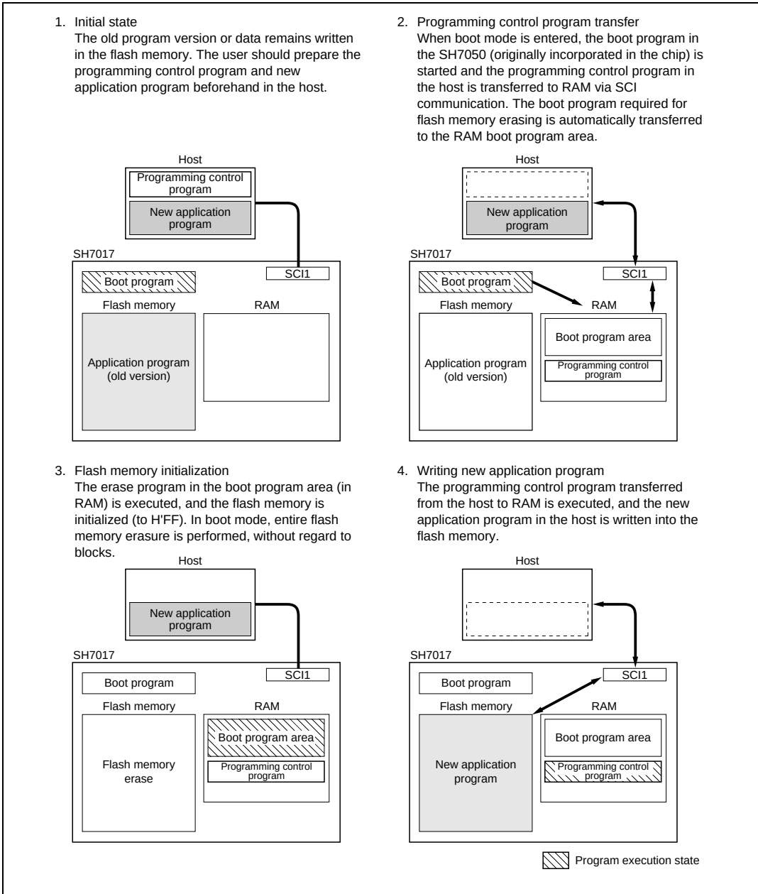
Figure 18.3 Boot Mode
