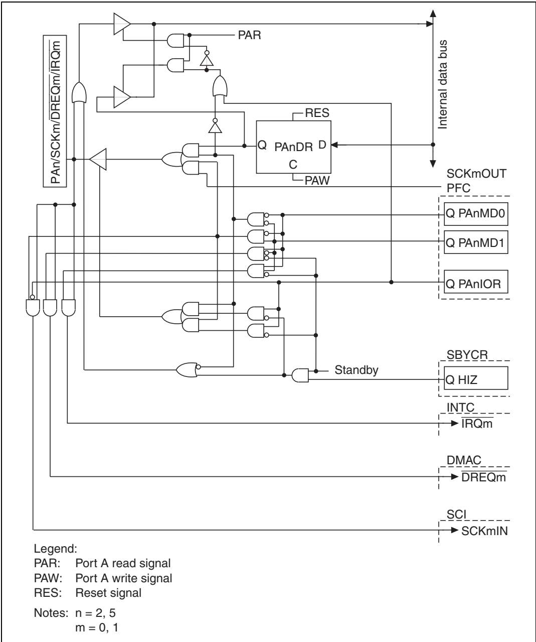
Figure B.2 PAn/SCKm/DREQm/TRQm Block Diagram
