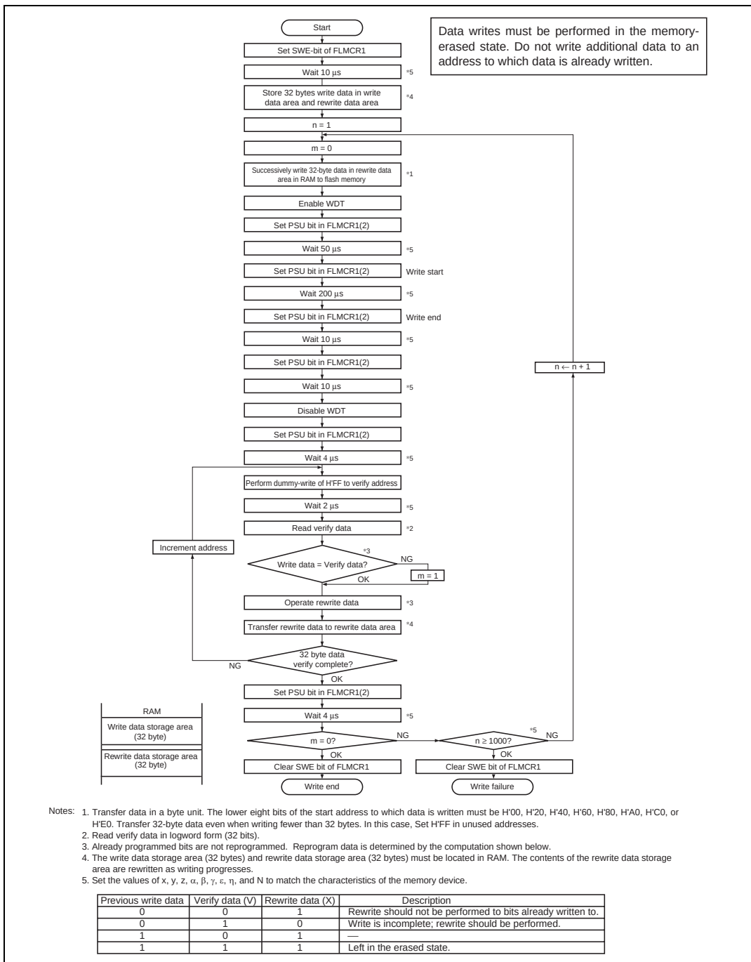
Figure 18.13 Program/Program-Verify Flowchart
