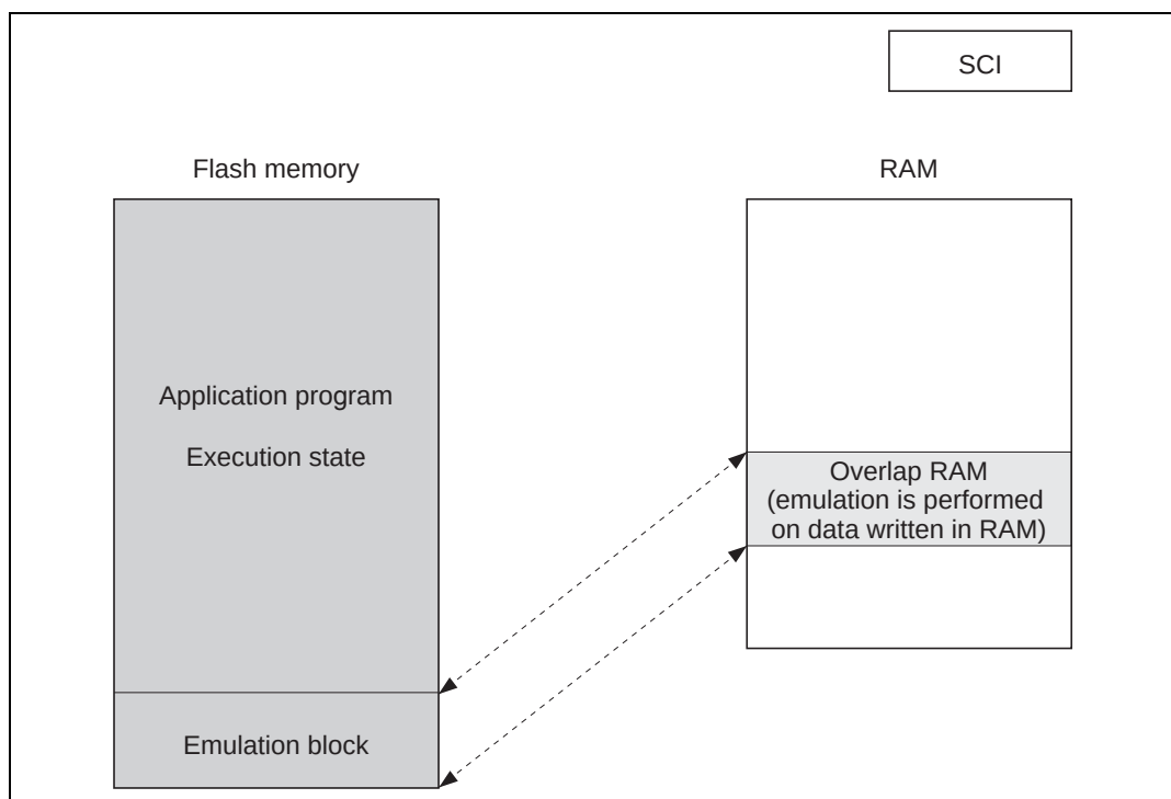
Figure 18.5 Emulation
