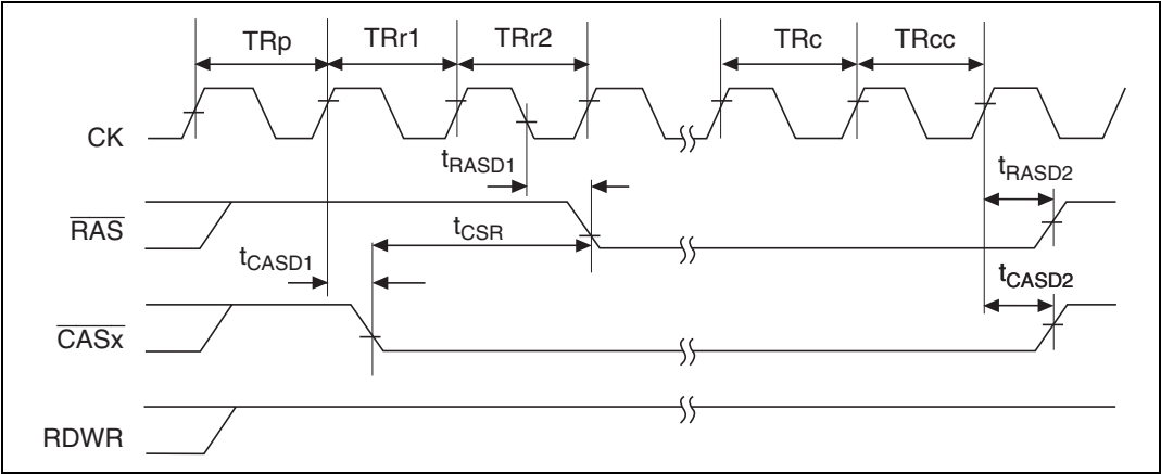
Figure 22.16 Self Refresh
