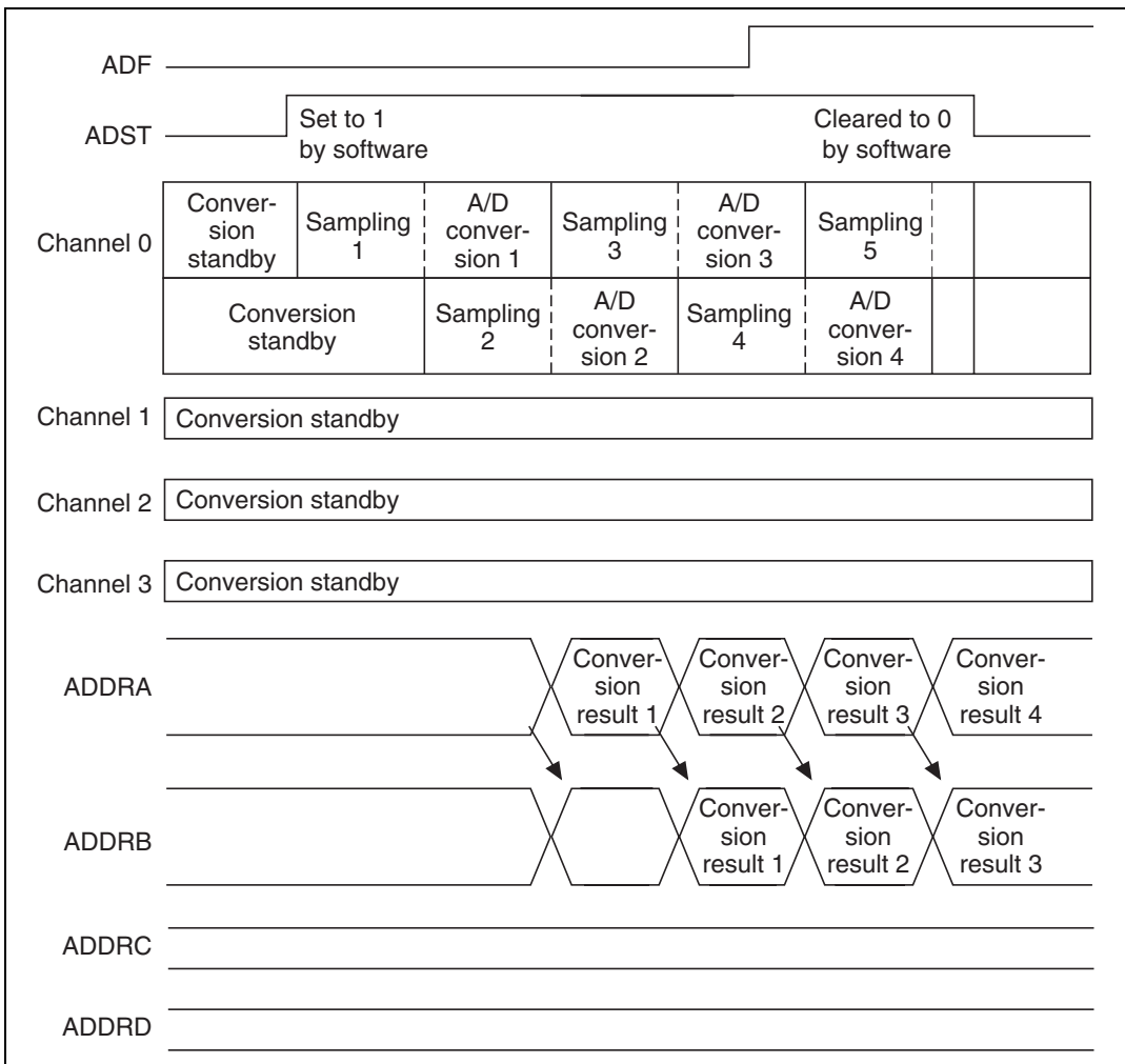
Figure 13.7 Buffer Operation Example (Select Scan Mode: Two-Stage One-Group Operation, When CH2 to CH0 = B'001)
