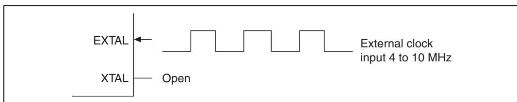
Figure 4.6 Example of External Clock Connection
