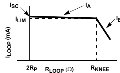
FIGURE 5. I_{LOOP} vs R_{LOOP} LOAD CHARACTERISTIC
