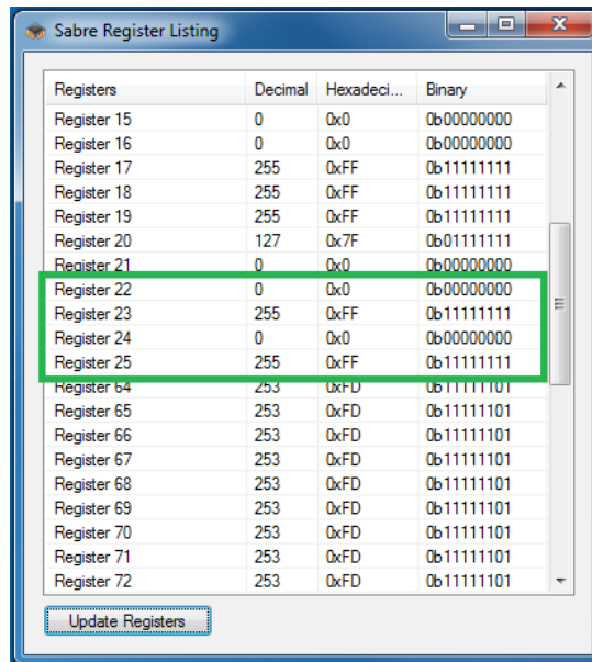
Figure 3. THD Compensation Registers in the register listing
