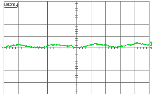
Fig. 14: Input reflected ripple current, i_s (10 mA/div.), measured through 10 \mu H at the source at full rated load current and V_{in} = 48 V. Refer to Fig. 12 for test setup. Time scale: 1 \mu s/div.
