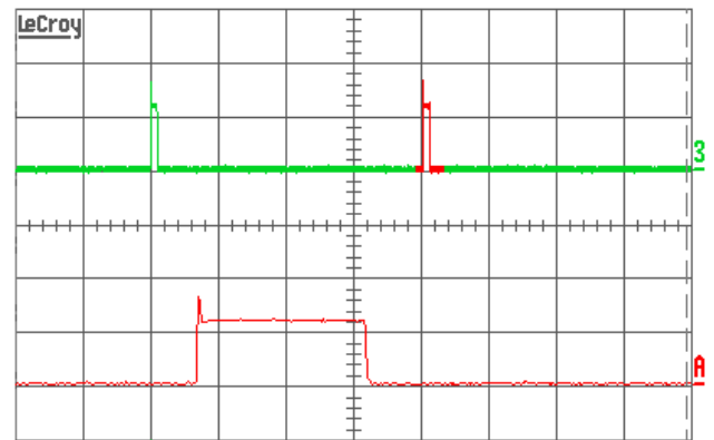
Fig. 16: Load current (top trace, 20 A/div., 50 ms/div.) into a 10 m\Omega short circuit during restart, at V_{in} = 48 V. Bottom trace (20 A/div., 2 ms/div.) is an expansion of the on-time portion of the top trace.
