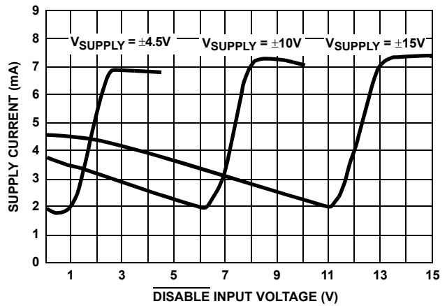
FIGURE 16. SUPPLY CURRENT vs \overline{DISABLE} INPUT VOLTAGE
