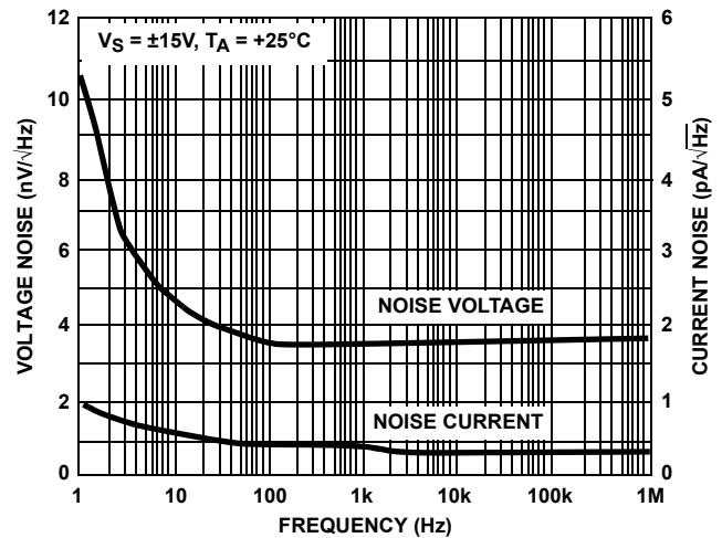
FIGURE 8. NOISE CHARACTERISTICS
