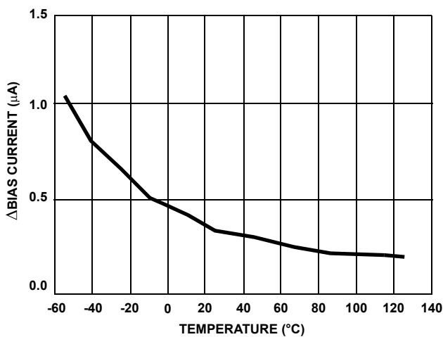
FIGURE 36. INPUT BIAS CURRENT CHANGE BETWEEN CHANNELS vs TEMPERATURE
