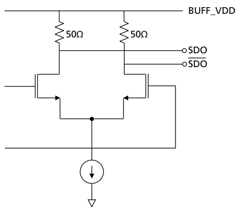
Figure 3-9: SDO/SDO-bar
