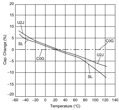
C0G/U2J/SL Characteristics
