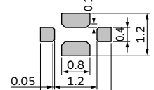
NFM18PS
