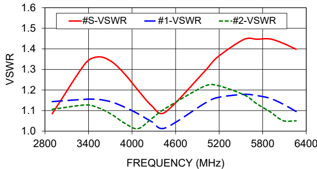
GP2X+ VSWR
