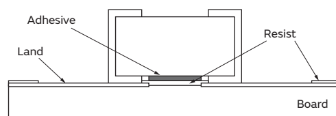
Cross Sectional View
