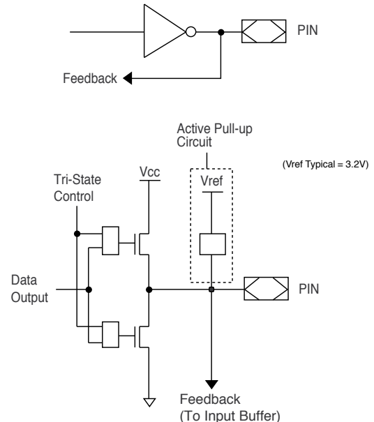
Typical Output
