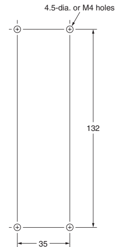
Panel Cutout Dimensions
