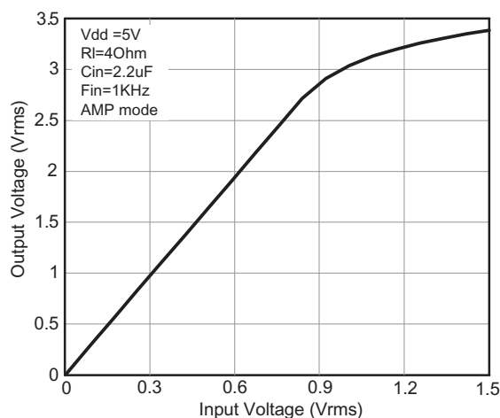
Figure 18. Input Voltage vs. Output Voltage
