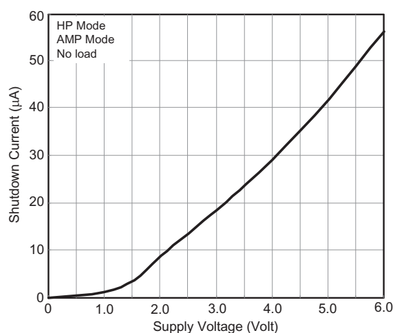
Figure 57. Shutdown Current vs. Supply Voltage
