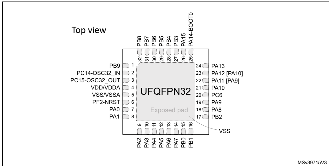
Figure 7. STM32G051KxU UFQFPN32 pinout
