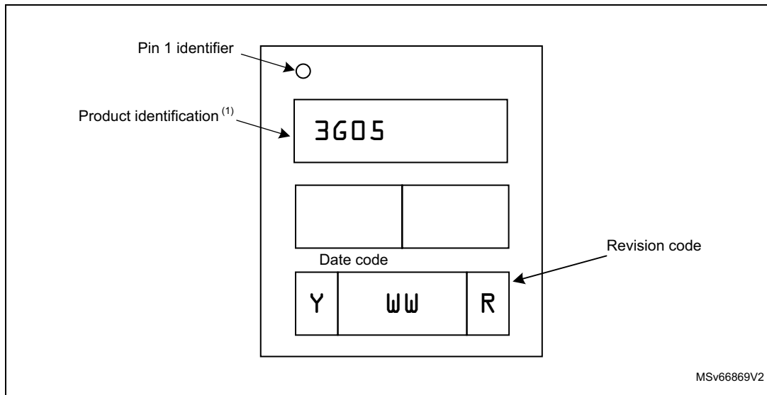
Figure 36. WLCSP20 package marking example
