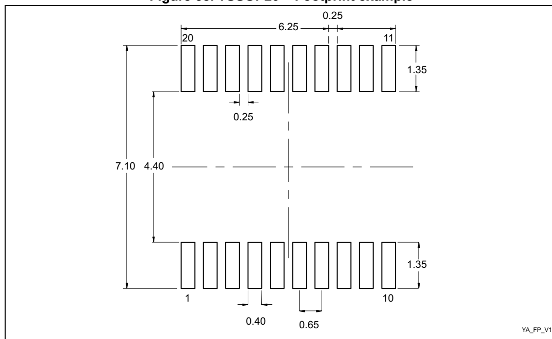
Figure 38. TSSOP20 – Footprint example
