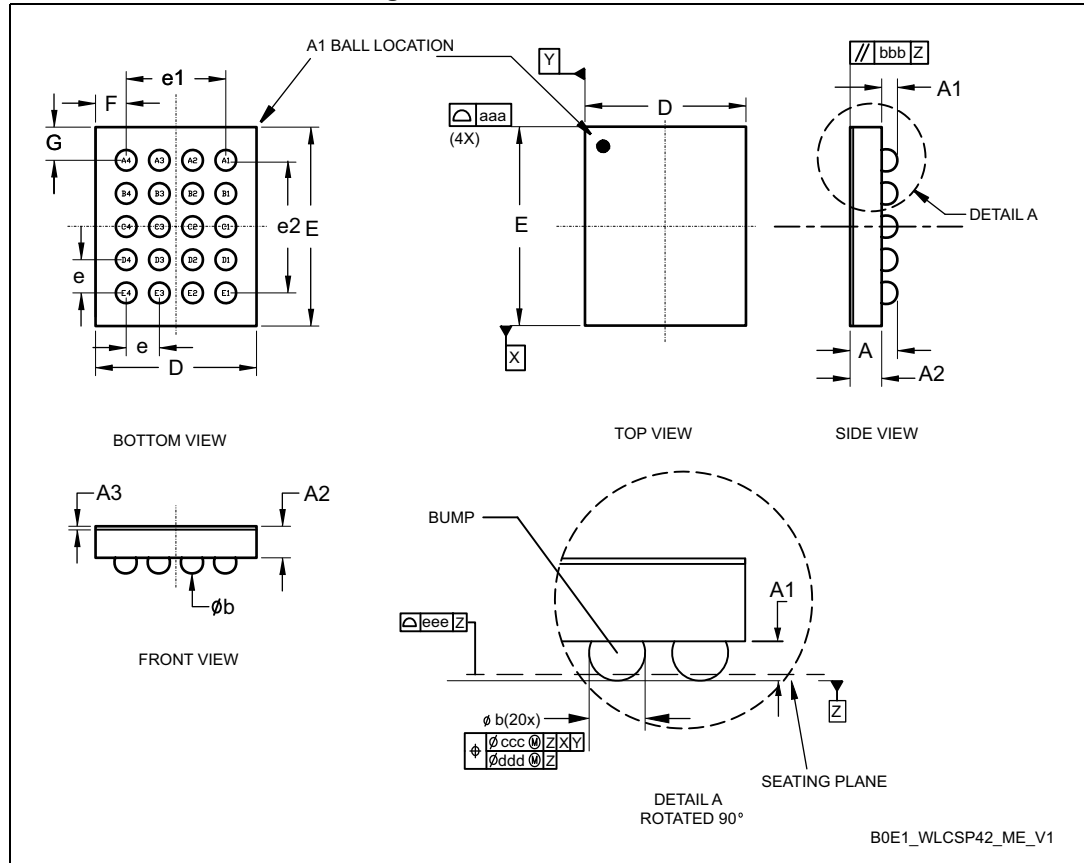
Figure 34. WLCSP20 - Outline
