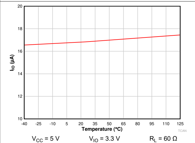
Figure 6-4. I_{IO} Standby vs Temperature
