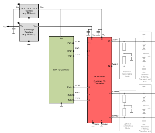
Simplified Schematics
