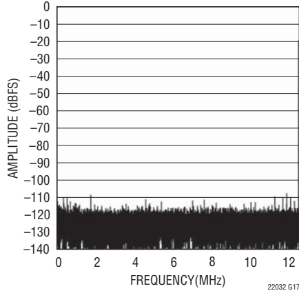
LTC2203: 32K Point FFT, f IN = 12.4MHz, -20dBFS, PGA = 0
