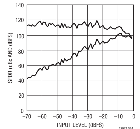
LTC2203: SFDR vs Input Level, f IN = 30.1MHz, PGA = 0, Dither "On"
