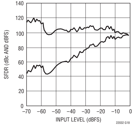
LTC2203: SFDR vs Input Level, f IN = 12.7MHz, PGA = 0, Dither "Off"
