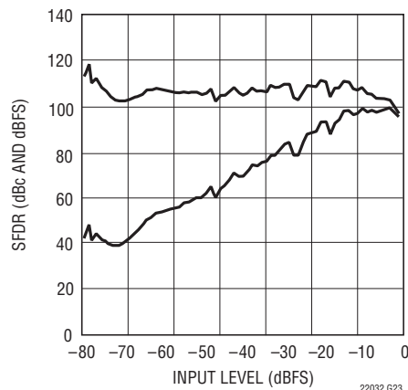
LTC2203: SFDR vs Input Level, f IN = 30.1MHz, PGA = 0, Dither "Off"
