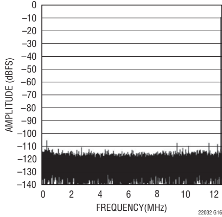
LTC2203: 32K Point FFT, f IN = 12.4MHz, -10dBFS, PGA = 0
