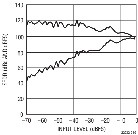
LTC2203: SFDR vs Input Level, f IN = 12.7MHz, PGA = 0, Dither "On"
