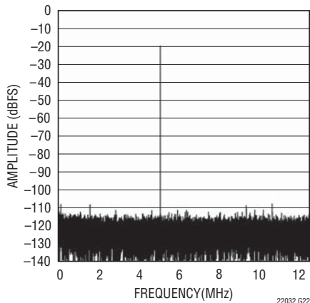
LTC2203: 32K Point FFT, f IN = 30MHz, -20dBFS, PGA = 1
