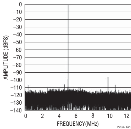
LTC2203: 32K Point FFT, f IN = 30MHz, -1dBFS, PGA = 1
