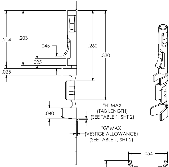
FIG 1 (CC03X-2830-01-X SHOWN)
