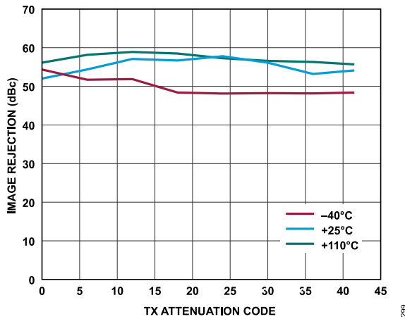
Figure 205. Transmitter Image Rejection vs. Transmitter Attenuation Code, Baseband Frequency = 18 MHz, Backoff = 0.2 dBFS, Initialization Calibration Only
