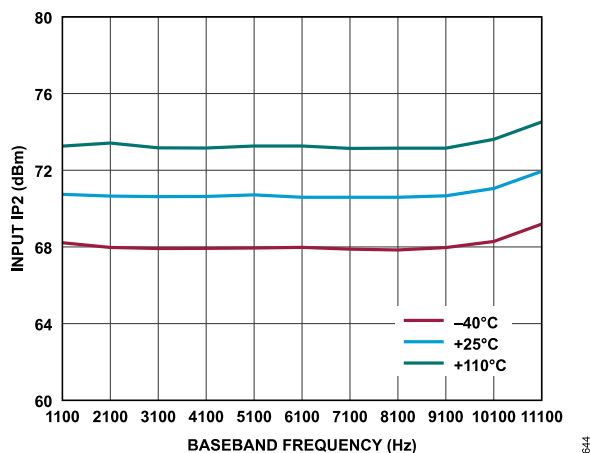
Figure 323. Receiver Input IP2 vs. Baseband Frequency, ADC = Low Power, f_1 = \text{Baseband Frequency} + 1 \text{ MHz} , f_2 = \text{Baseband Frequency} + 2 \text{ MHz} , Gain Index = 255, First-Order TIA with f_{3dB} = 4 \text{ MHz} , P_{OUT} = -6.6 \text{ dBFS}
