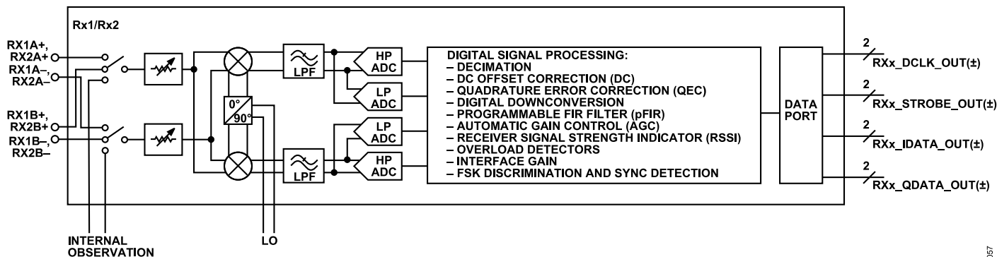
Figure 361. Receiver Architecture
