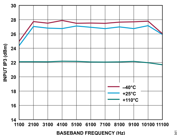
Figure 320. Receiver Input IP3 vs. Baseband Frequency, ADC = High Performance, f_1 = \text{Baseband Frequency} + 1 \text{ MHz} , f_2 = \text{Baseband Frequency} + 2 \text{ MHz} , Gain Index = 255, First-Order TIA with f_{1dB} = 4 \text{ MHz} , P_{OUT} = -12.6 \text{ dBFS} at -40^\circ\text{C} and +25^\circ\text{C} , P_{OUT} = -15.6 \text{ dBFS} at +110^\circ\text{C}
