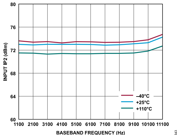
Figure 322. Receiver Input IP2 vs. Baseband Frequency, ADC = High Performance, f_1 = \text{Baseband Frequency} + 1 \text{ MHz} , f_2 = \text{Baseband Frequency} + 2 \text{ MHz} , Gain Index = 255, First-Order TIA with f_{3dB} = 4 \text{ MHz} , P_{OUT} = -6.6 \text{ dBFS}
