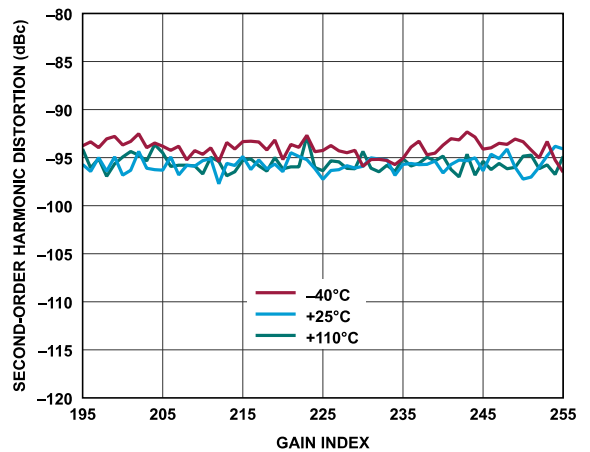
Figure 243. Receiver Second-Order Harmonic Distortion vs. Gain Index, Baseband Frequency = 2.1 kHz, ADC = Low Power
