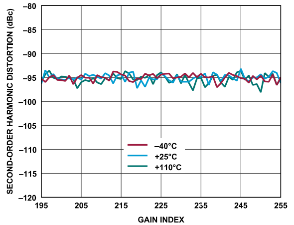
Figure 241. Receiver Second-Order Harmonic Distortion vs. Gain Index, Baseband Frequency = 2.1 kHz, ADC = High Performance
