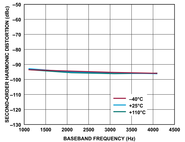
Figure 242. Receiver Second-Order Harmonic Distortion vs. Baseband Frequency, Gain Index = 255, ADC = High Performance
