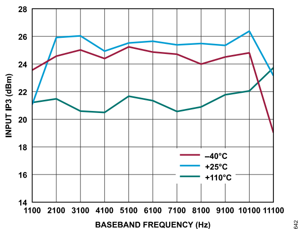
Figure 321. Receiver Input IP3 vs. Baseband Frequency, ADC = Low Power, f_1 = \text{Baseband Frequency} + 1 \text{ MHz} , f_2 = \text{Baseband Frequency} + 2 \text{ MHz} , Gain Index = 255, First-Order TIA with f_{1dB} = 4 \text{ MHz} , P_{OUT} = -12.6 \text{ dBFS} at -40^\circ\text{C} and +25^\circ\text{C} , P_{OUT} = -15.6 \text{ dBFS} at +110^\circ\text{C}
