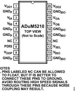
Figure 3. ADuM5210 Pin Configuration
