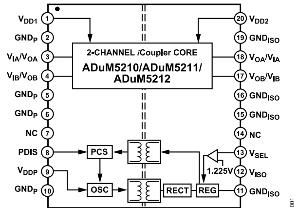
Figure 1. ADuM5210/ADuM5211/ADuM5212
