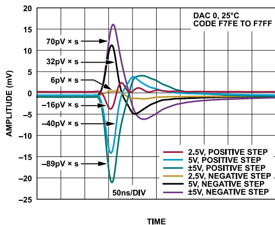
Figure 53. Digital-to-Analog Glitch
