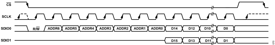
Figure 93. Dual SPI Mode
