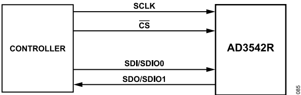
Figure 91. Single SPI (Classic SPI) Connection
