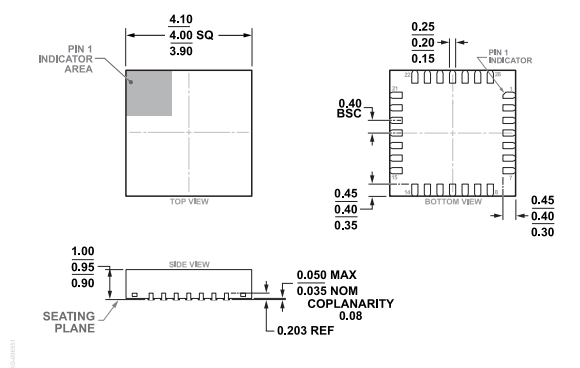
Figure 101. 28-Lead Lead Frame Chip Package [LFCSP] 4 mm × 4 mm Body and 0.95 mm Package Height (CP-28-15) Dimensions shown in millimeters
