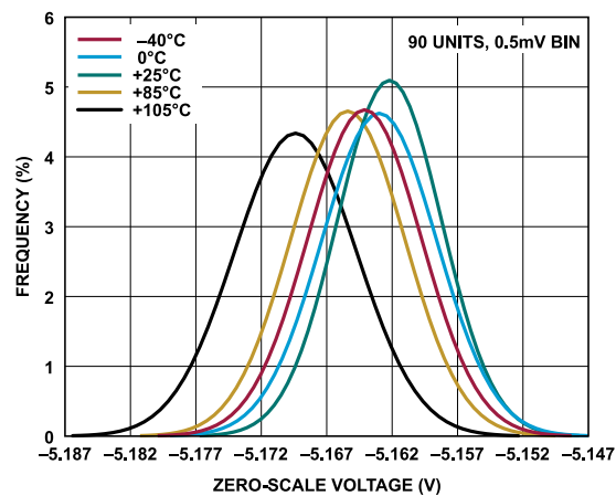
Figure 44. Zero-Scale Voltage Distribution, -5 V to +5 V Range
