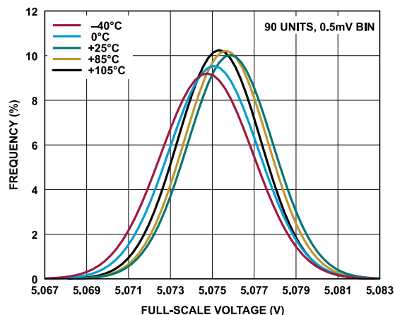
Figure 47. Full-Scale Voltage Distribution, 0 V to 5 V Range
