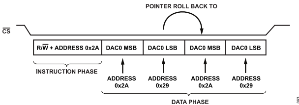
Figure 87. Looping Enabled with Address Descending and STREAM\_MODE = 2
