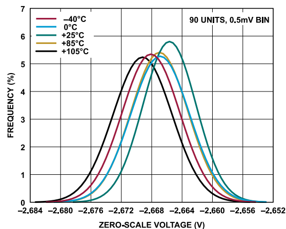
Figure 45. Zero-Scale Voltage Distribution, -2.5 V to +7.5 V Range
