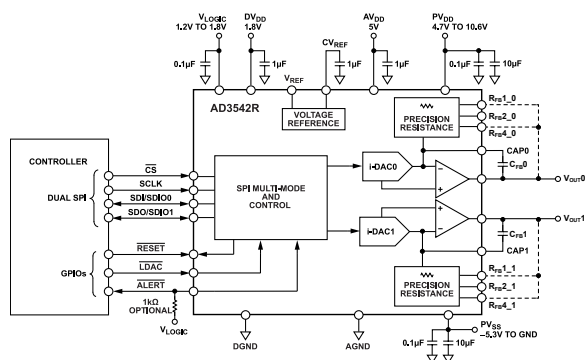
Figure 99. Recommended Application Circuit
