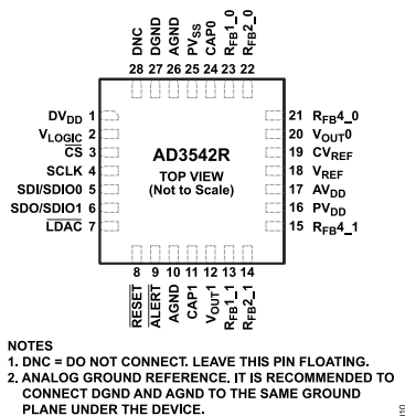
Figure 10. Pin Configuration
