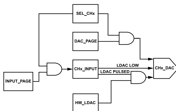
Figure 97. DAC Data Flow Between Registers
