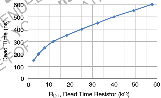
Figure 31. Dead Time vs. R_{DT}
