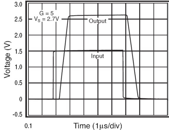
Figure 23. Overdrive Recovery
