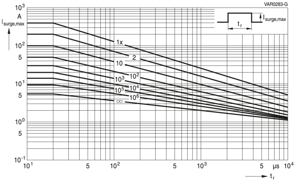
CT1210K17AUTOG
